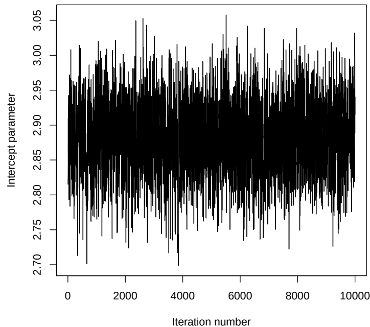
Figure 2: Trace plot for the intercept parameter, \phi , in the alcohol, obesity and hypertension example.
