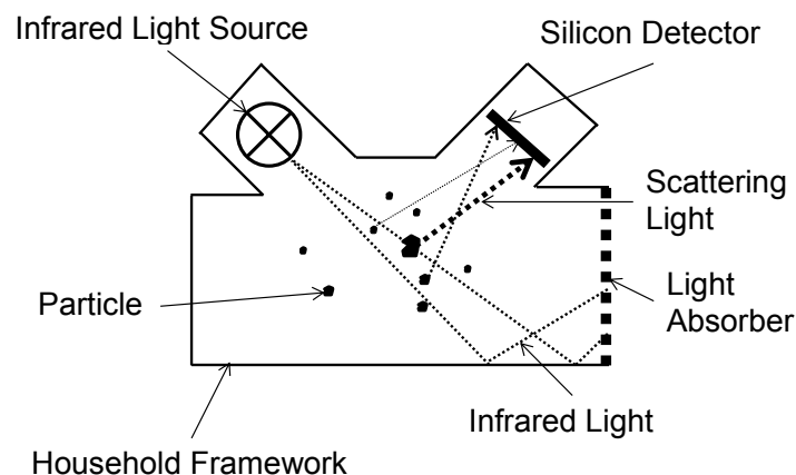
Figure 6. Basic Nephelometer.
