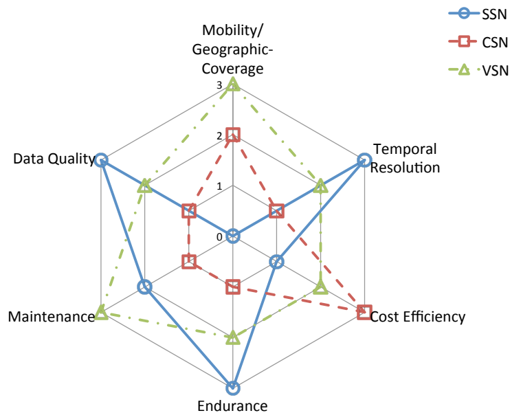
Figure 11. Grading result of the six major comparison properties in Static Sensor Network (SSN), Community Sensor Network (CSN) and Vehicle Sensor Network (VSN) ('0' means 'None'; '1' means 'Low/Short/Inconvenient'; '2' means 'Medium' and '3' means 'High/Long/Convenient').
