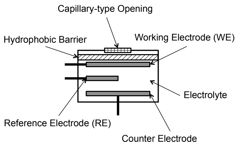
Figure 4. Basic Electrochemical Sensor.
