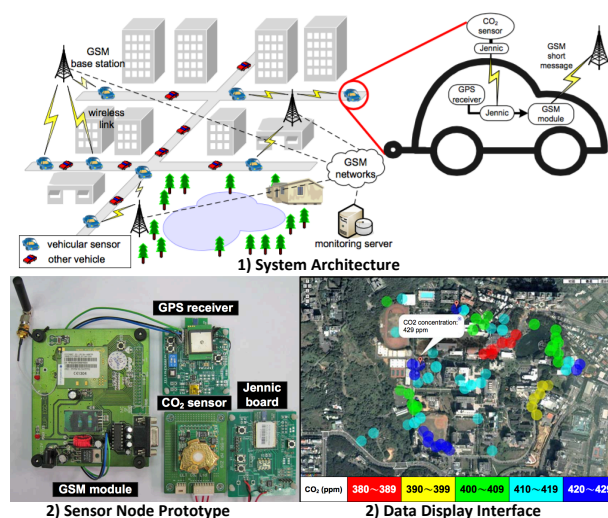
Figure 10. Example of the Vehicle Sensor Network (VSN) system architecture and prototype. Figures are adapted from [98].
