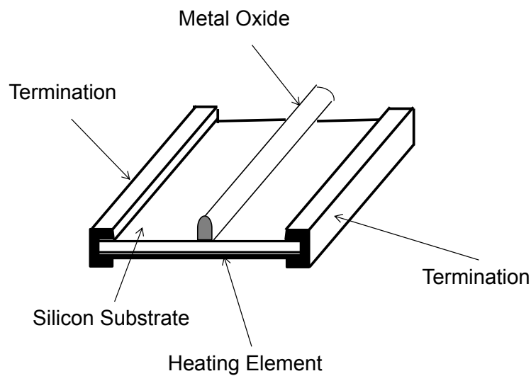
Figure 3. Chip-type Sensor.
