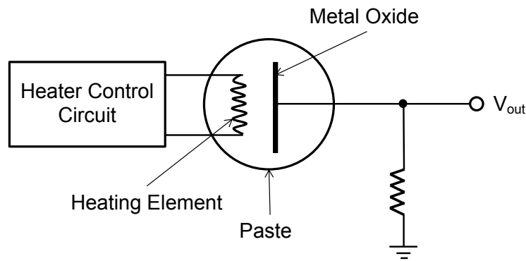
Figure 2. Bead-type sensor.
