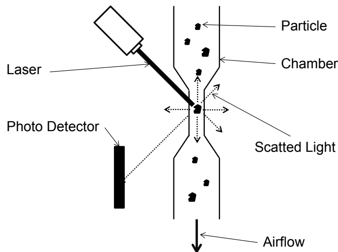
Figure 5. Basic Light Scattering Particle Counter.
