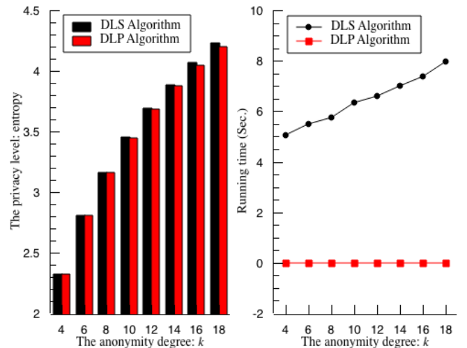
Fig.7: Entropy and running times under Scenario C
