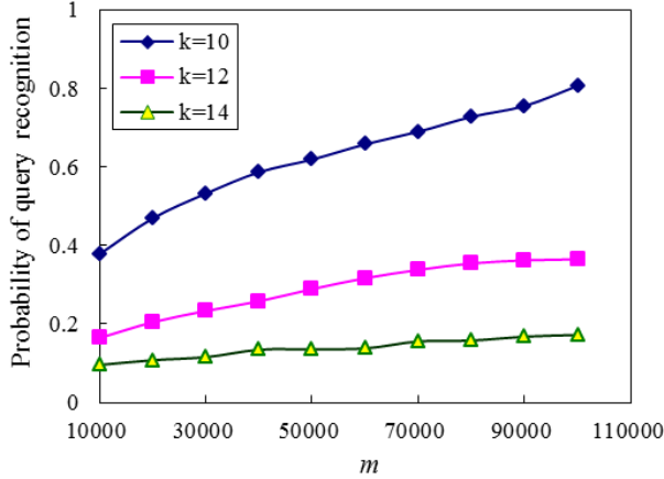
Fig.3: The probability of query recognition achieved in different anonymity degree k under Scenario-1.2.
