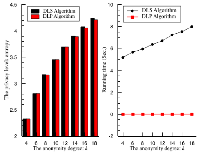
Fig.6: Entropy and running times under Scenario B
