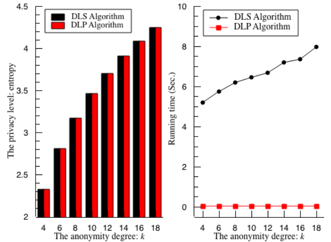
Fig.5: Entropy and running times under Scenario A
