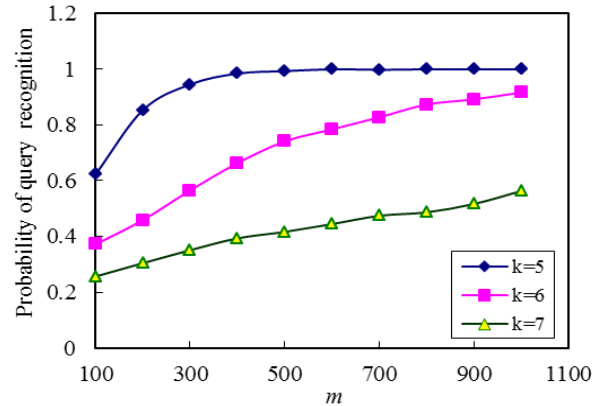
Fig.2: The probability of query recognition achieved with different anonymity degrees k under Scenario-1.1.
