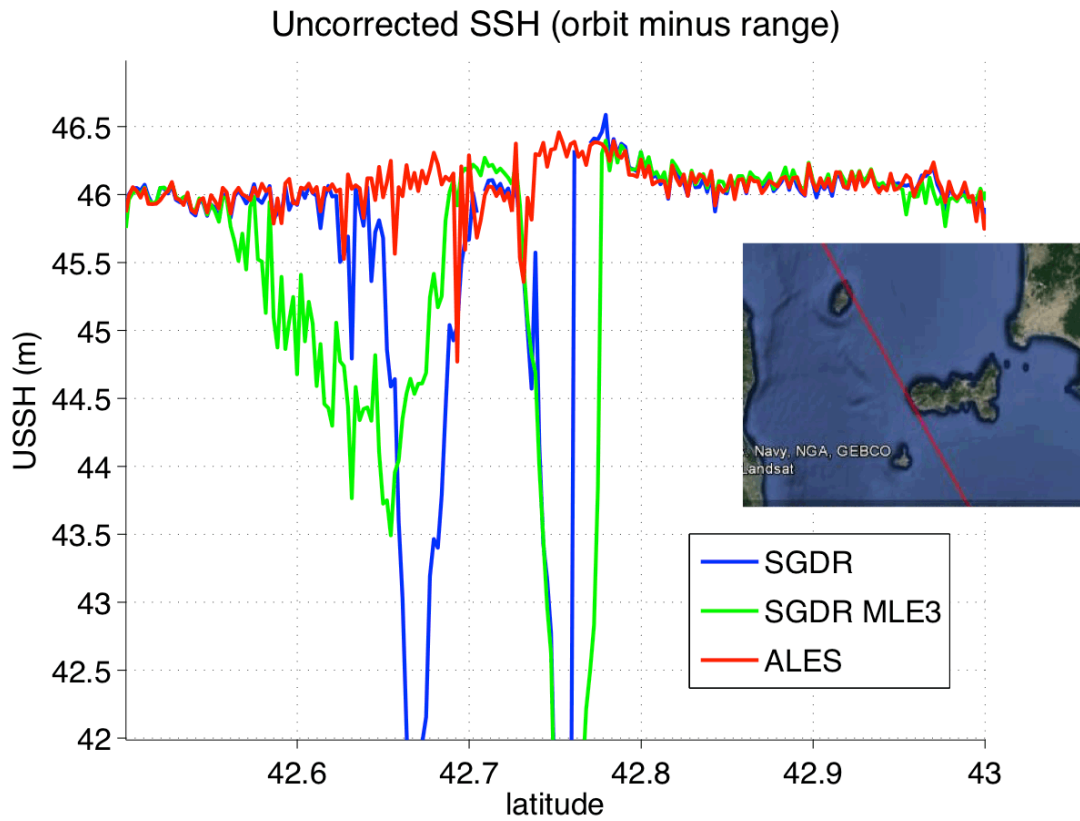
Figure 5 – Example of improved retrieval of sea level (here labelled as sea surface height or SSH) close to the coast via a specialized algorithm. The inset shows a map of Jason-2 descending pass 0044 (red track) in the vicinity of Elba Island in the Mediterranean Sea. The line plots show the 20-Hz uncorrected SSH (i.e. orbital altitude of the satellite minus retracked range) measured during the overpass of that ground track during orbital cycle 252 (at 13:40 on 7 May 2015) using three different retrackerers: the standard Brown 4-parameter available in the Sensor Geophysical Data Records ('SGDR', in blue), the 3-parameter Maximum Likelihood Estimator also in the SGDR ('SGDR MLE3', in green), and the ALES retracker (Passaro et al., 2014). The ALES estimates are much less affected by the proximity to the Elba Island coast within 42.65°N and 42.8°N.
