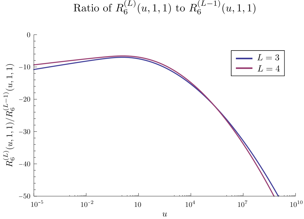
Figure 3. The successive ratios R_6^{(L)}/R_6^{(L-1)} on the line (u, 1, 1) .
