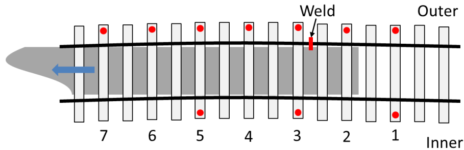
Figure 4: Site layout prior to renewal showing the approximate extent of the wet bed (in grey) and the vertical geophones (red circles). The arrow indicates the direction of travel.
