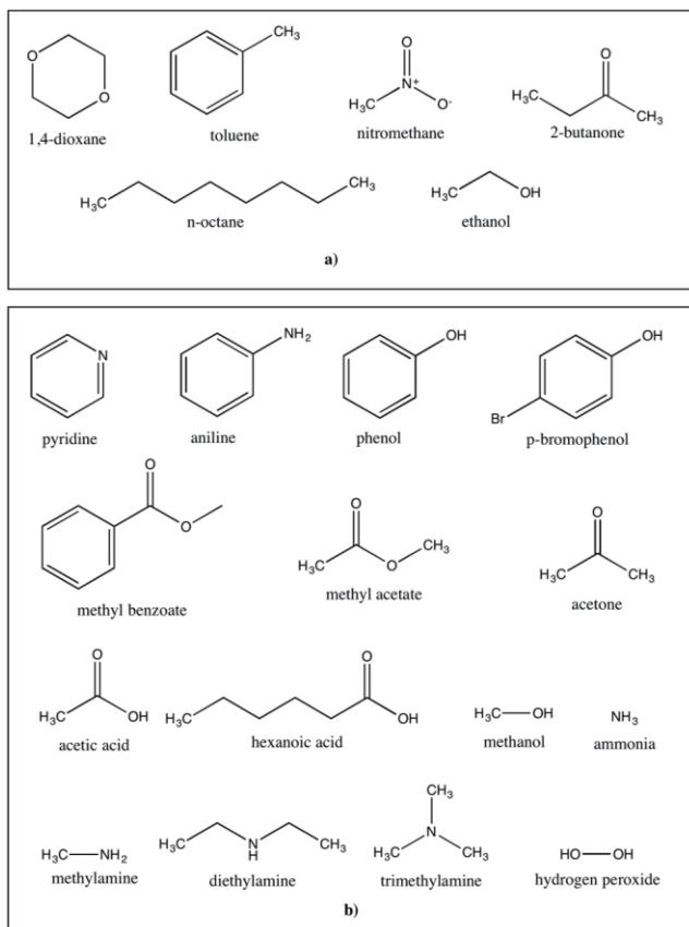
Figure 1. The structures of small molecules selected in this study. a) Data set of small molecules for toluene, chloroform, acetonitrile and DMSO solvent. b) Data set of additional small molecules for toluene and chloroform solvent.
