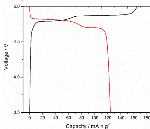
Fig. 1 Voltage profile during the first cycle of LiCoPO 4 conducted in a lithium half-cell (standard Swagelok cell) at 0.1 C showing plateaux corresponding to conversion of phase A ( \approx LiCoPO 4 ) to B ( \approx Li 2/3 CoPO 4 ) and B to C ( \approx CoPO 4 ).
