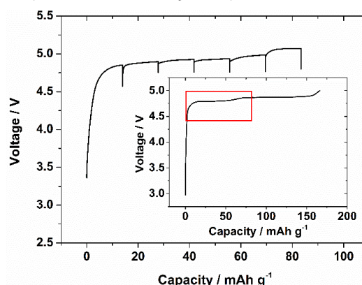
Fig. 5 Voltage/charge profile of \text{LiCoPO}_4 collected during GITT lithium extraction in the in situ cell with pulse charges for 10 min at 0.5C and 30 min relaxations. Inset shows the charge profile collected in a standard Swagelok cell (from Fig. 1) with the red box showing the equivalent charge region.
