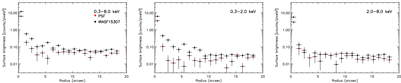
Figure 4. Left: Surface brightness profile in the 0.3–8.0 keV energy range of the Chandra PSF (red) and the observed emission (black). Middle: Same but for the 0.3–2.0 keV energy range. Right: Same but for the 2.0–8.0 keV energy range. These plots show that IRAS F15307+3252 is indeed extended at X-ray wavelengths, but only in the soft 0.3–2.0 keV band.
