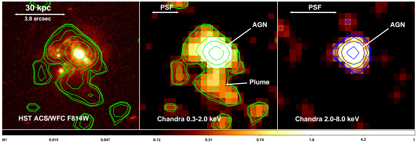
Figure 3. Small-scale image of IRAS F15307+3252. Left: HST ACS/WFC image of the central regions of IRAS F15307+3252 obtained with the F814W filter. Middle: Chandra image in the soft X-ray band (0.3 – 2.0 keV), smoothed with a gaussian function of 2 arcsec. The green contours highlight the detected emission in the 0.3 – 2.0 keV band, starting at a 2\sigma level. These contours are also overplotted in the left panel. They highlight the same small, plume-like extended emission to the south as in Fig. 1. Right: Chandra image in the hard X-ray band (2.0 – 8.0 keV), smoothed with a gaussian function of 2 arcsec and showing the AGN point source. The blue contours show the hard X-ray band emission (2.0 – 8.0 keV), also starting at a 2\sigma level. The color bar indicates the number of counts per pixel for the 0.3 – 2.0 keV image.
