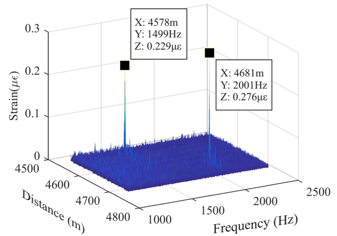
Fig. 2. Frequency components present along a 300m stretch of the sensing fibre between 4500m and 4800m.
