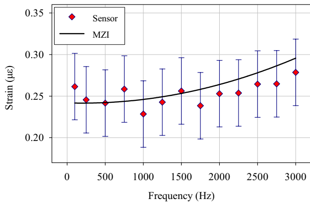
Fig. 4. Frequency response of the large PZT measured by the distributed sensor (red data-points) and MZI (solid-line).
