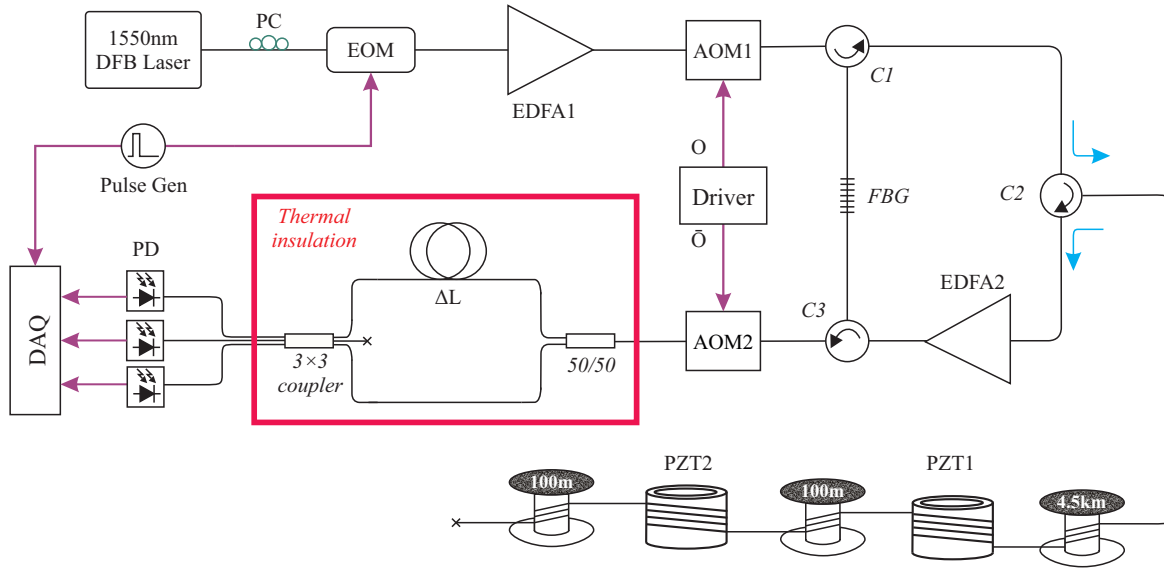
Fig. 1. Experimental setup. DFB: distributed feedback, PC: polarization controller, EOM: Electro-optic modulator, EDFA: erbium-doped fibre amplifier, AOM: Acousto-optic modulator, C: circulator, FBG: fibre Bragg grating, PD: photodetector, DAQ: Data Acquisition System.
