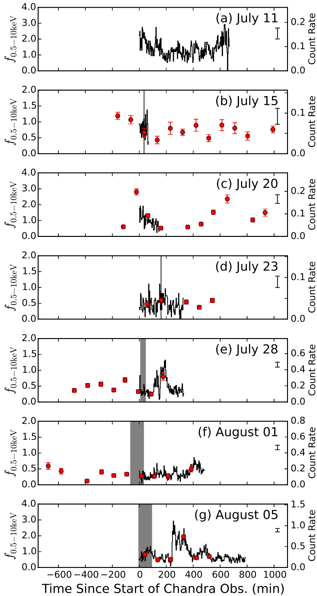
Figure 2. X-ray Light curves of seven Chandra observations binned by 3 min (black solid lines), with typical error bars illustrated in the top right of each panel. X-ray fluxes from \approx 1 -2 ks Swift snapshots are overplotted (red circles). Shaded regions mark when the VLA observed. X-ray fluxes are from 0.5-10 keV, in units of 10^{-11} erg s^{-1} cm^{-2} (see left vertical axes), and count rates for the Chandra observations are listed on the right vertical axes. The x-axis is referenced to the start time of each Chandra observation (see Table 1; times from all telescopes are barycentered).
