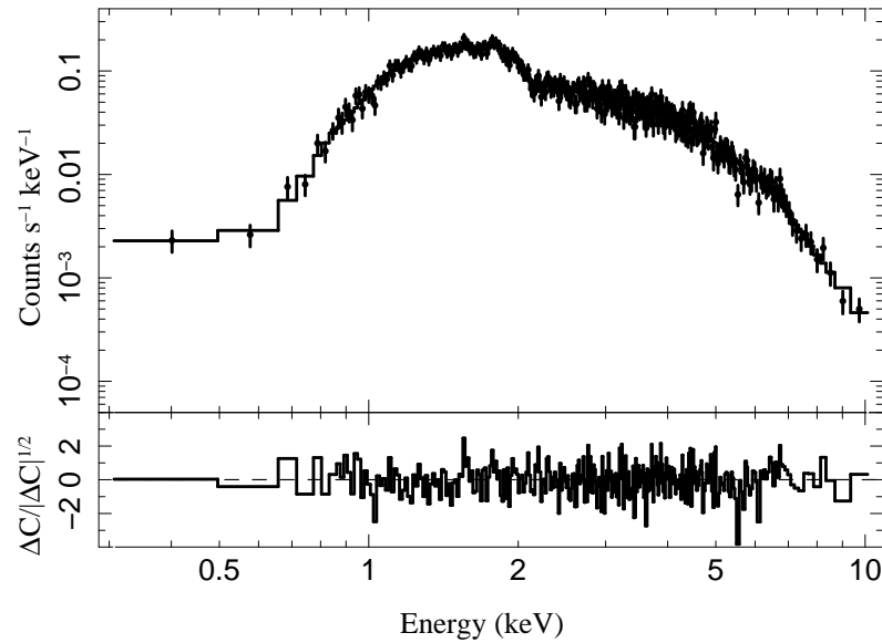
Figure A2. Chandra X-ray spectrum from August 5, as an example of the quality of our spectral fits.
