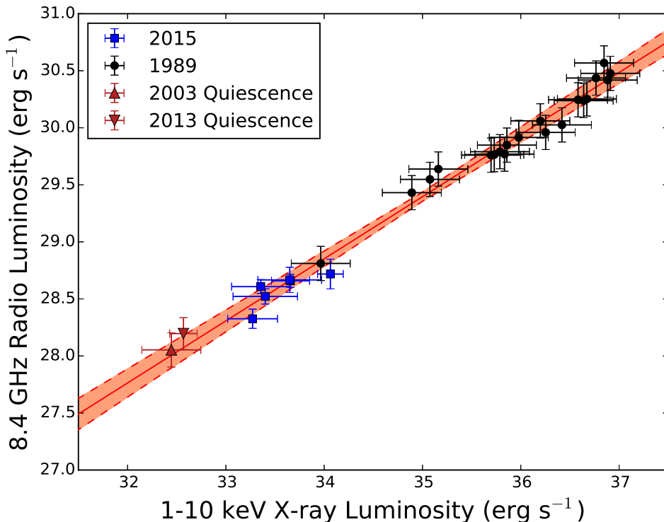
Figure 7. The radio/X-ray luminosity correlation for V404 Cygni. Blue squares show observations from our 2015 campaign, including the simultaneous VLBA and Swift observations on July 11. Black circles show data from the 1989 decay (Corbel et al. 2008), and the red triangles show two pre-outburst epochs: 2003 (Corbel et al. 2008; Hynes et al. 2009) and 2013 (Rana et al. 2016). The red solid line and shaded region shows the best-fit to the radio/X-ray correlation ( L_R \propto L_X^{0.54} ) and the 1\sigma uncertainty.
