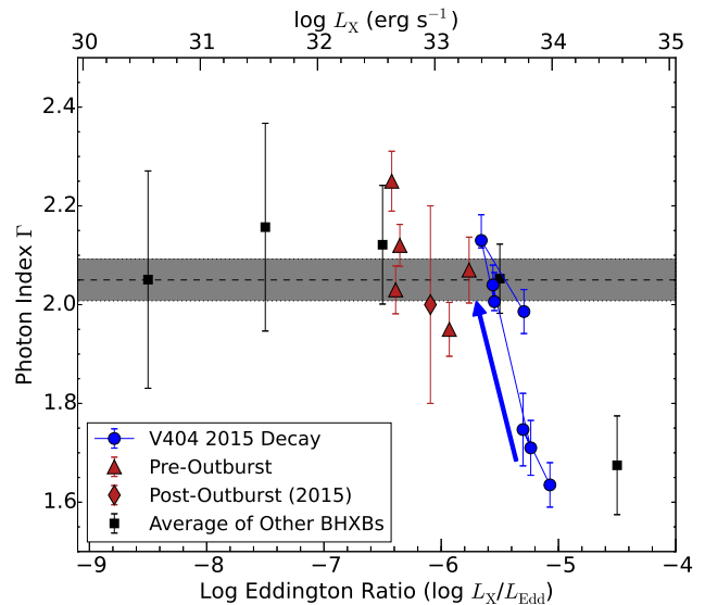
Figure 8. The X-ray spectral evolution of V404 Cygni as function of Eddington ratio ( L_X/L_{\text{Edd}} , where L_X , which is displayed along the top axis, is calculated from 0.5-10 keV). Blue circles represent observations from our 2015 decay, with the blue solid lines connecting the data points to illustrate the evolution with time (following the direction of the blue arrow). Red triangles show spectral fits from pre-outburst observations compiled from Reynolds et al. (2014) and Rana et al. (2016), the red diamond represents a Chandra observation from 2015 November (Tomsick et al. 2015), and black squares represent the average photon indices of ten quiescent BHXBs binned by Eddington ratio, from Plotkin et al. (2013). The X-ray spectral softening occurs over a narrow range in Eddington ratio (from 10^{-5.1} to 10^{-5.6} ), which is more luminous than the average pre-outburst Eddington ratio ( 10^{-6.2} ; Bernardini & Cackett 2014). The dashed line and grey shaded region illustrate the average \Gamma and 1\sigma confidence interval for V404 Cygni pre-outburst (from Reynolds et al. 2014).
