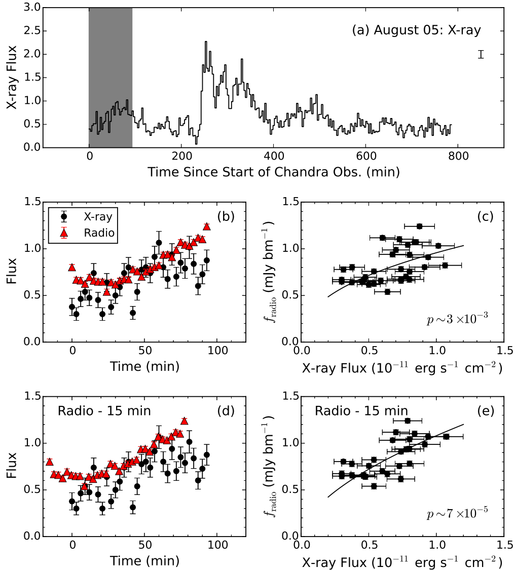
Figure 5. (a) The hard (1–10 keV) Chandra X-ray light curve from August 5 (binned by 3 min), with the shaded region denoting the time period with strictly simultaneous VLA observations. A typical error bar is illustrated in the top right corner. (b) X-ray (black circles) and radio (red triangles) light curves during the period of strict simultaneity. (c) Radio vs. X-ray emission. A Pearson correlation test indicates a (marginal) positive correlation at the p \approx 3 \times 10^{-3} level. The black solid shown shows the best-fit radio/X-ray correlation during the 93 min of strict simultaneity ( L_{\text{R}} \propto L_{\text{X}}^{0.4 \pm 0.2} ). (d) Same as panel (b), except with the radio data delayed by 15 min. (e) Same as panel (c), except with X-ray light curves re-extracted after factoring in the 15 min radio delay. After correcting for the time delay, a Pearson correlation test indicates a stronger correlation ( p \approx 7 \times 10^{-5} ), and L_{\text{R}} \propto L_{\text{X}}^{0.6 \pm 0.2} . All X-ray fluxes are from 1–10 keV (in units of 10^{-11} erg \text{s}^{-1} \text{cm}^{-2} ), and all radio flux densities are at 8.4 GHz (in units of \text{mJy } \text{bm}^{-1} ); the normalizations of the radio and X-ray light curves in panels (b) and (d) correspond to the aforementioned units.
