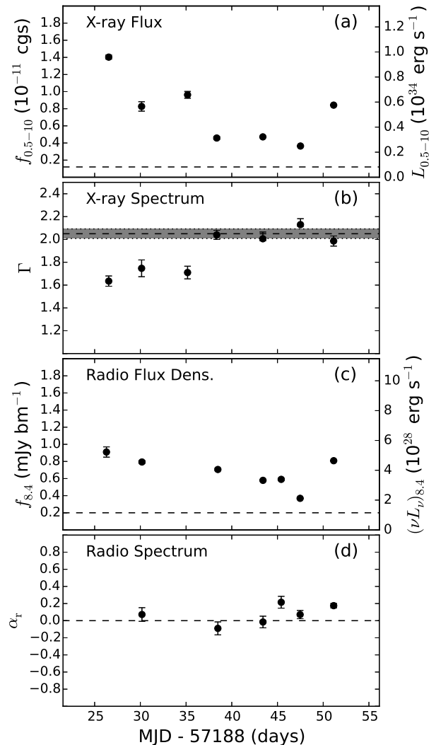
Figure 1. (a) Chandra X-ray light curve during our three-week campaign. Unabsorbed X-ray fluxes (luminosities) from 0.5-10 keV are labeled on the left (right) vertical axis. The dashed line illustrates the average pre-outburst X-ray flux (Bernardini & Cackett 2014) (b) Evolution of the X-ray photon index. The dashed line and gray shaded region denote the pre-outburst \Gamma and 1\sigma uncertainty from Reynolds et al. (2014). (c) Interpolated radio flux density light curve at 8.4 GHz (see left vertical axis); corresponding luminosities at 8.4 GHz are labeled on the right vertical axis, and the dashed line shows the pre-outburst radio flux density (Corbel et al. 2008). (d) Radio spectral index \alpha_{\text{r}} (we do not have radio spectral constraints from the July 11 VLBA observation). The dashed line marks a flat radio spectrum for reference. In all panels, the time axis is referenced to the discovery date of the outburst (2015 June 15).
