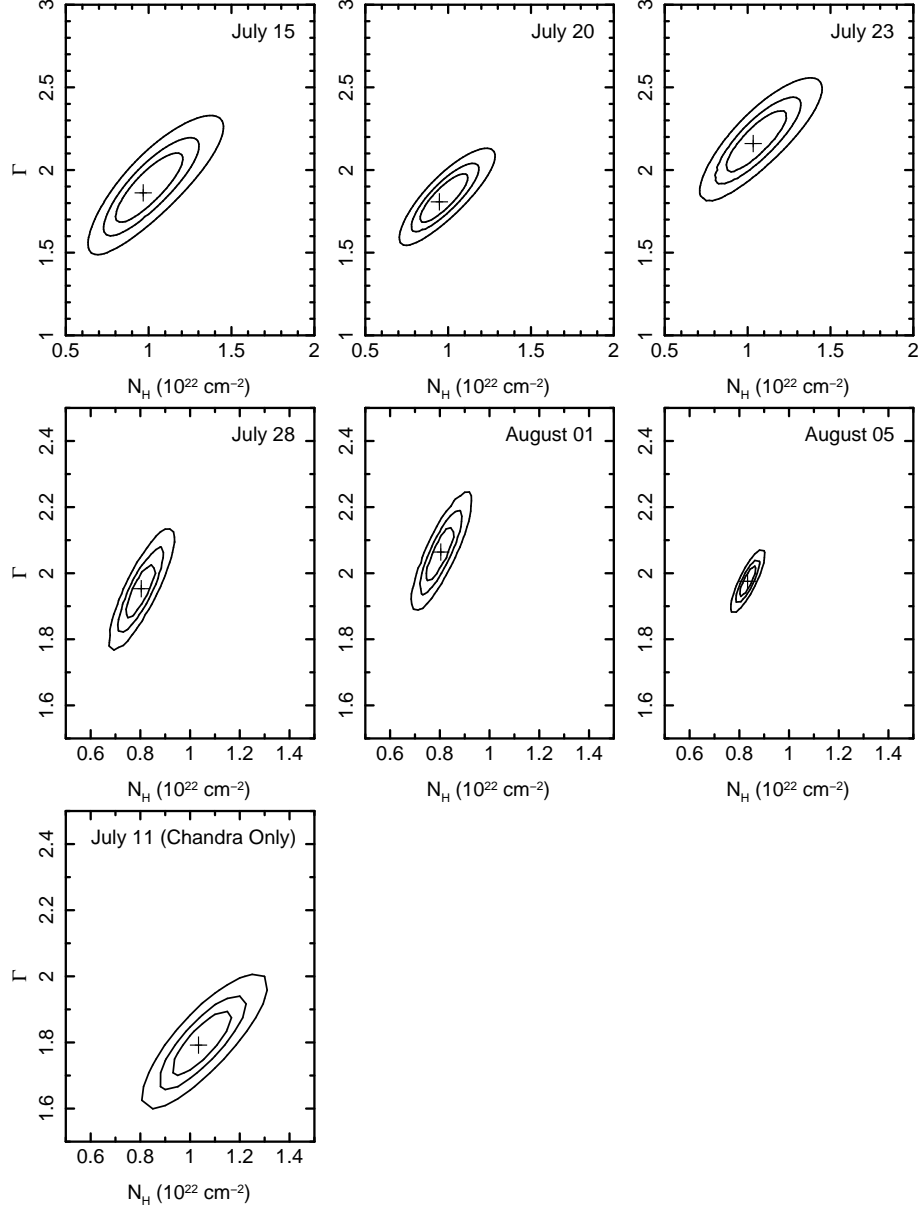
Figure A1. Confidence contour maps of joint spectral fits to the Chandra and Swift observations for the photon index ( \Gamma ) and the column density ( N_{\text{H}} ), when allowing N_{\text{H}} to vary as a free parameter on each epoch. Contours denote 68, 90, and 99% confidence intervals (corresponding to changes in the Cash statistic of \Delta C = 2.3, 4.6, and 9.2, respectively, for two parameters of interest). The final panel for July 11 does not include Swift data. Note the different axis scales for the top row, and that because we allow N_{\text{H}} to vary during each epoch, the errors illustrated here are larger than those listed in Table 3.
