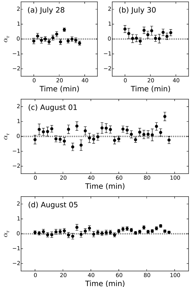
Figure 4. Variation of radio spectral index with time for the four longest radio epochs (binned by 3 min). The dotted lines mark \alpha_r = 0 for reference. The x-axis is referenced to the beginning of each VLA observation.
