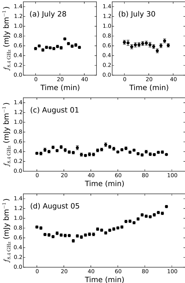
Figure 3. Radio light curves for the four epochs with the longest amount of radio coverage, binned by 3 min. The x-axis is referenced to the start time of each VLA observation.
