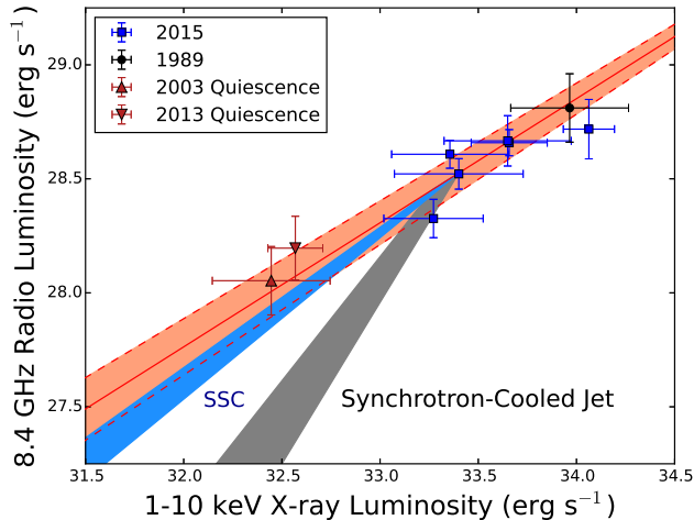
Figure 9. The radio/X-ray luminosity correlation from Figure 7, zoomed in on the 2015 data. Symbols have the same meaning as in Figure 7. The gray shaded region shows the predicted path V404 Cygni would take through the radio/X-ray plane if the X-ray spectral softening signifies a switch to synchrotron-cooled X-ray emission in quiescence, a scenario that is inconsistent with the pre-outburst radio luminosity. The light blue shaded region illustrates the path if the X-rays switch to SSC emission with synchrotron cooled seed photons.
