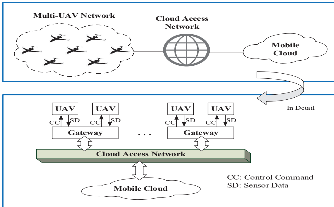
Fig. 3. The Architecture of a Multi-UAV Network Relying on a Cloud Control System.
