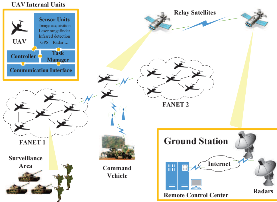
Fig. 1. Multi-UAV network architecture and necessary UAV internal units. Specifically, both the small and mini drones should be equipped with sensor units, control and management units, and communication units in order to fulfil certain tasks. Except for some essential sensors, such as the gyroscope, GPS, radar, etc. the drones carry specific sensors, depending on their particular missions. Moreover, the control and management units are responsible for the stable operation and the collaboration of each part. The communication units are composed of multiple modules configured by various protocols, such as IEEE 802.11, IEEE 802.15, LTE, etc. in order to support different communication scenarios. [5].
