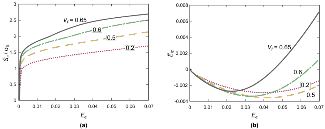
Figure 10: Predictions of the (a) \bar{S}_e / \sigma_0 - \bar{E}_e response under uniaxial compressive ( \eta = 1/3 ) and (b) corresponding strain paths in \bar{E}_m - \bar{E}_e space for the FCC unit cell with particle volume fractions in the range 0.2 \leq V_f \leq 0.65 and initial matrix porosity f_0 = 0.1 .
