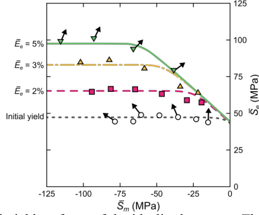
Figure 4: The measured yield surfaces of the idealised cermet. The initial yield surface and the evolution of the surface for 3 additional values of the effective strain \bar{E}_e are included. The plastic strain rate vectors are included for selected loading points with the \dot{\bar{E}}_e and \dot{\bar{E}}_m axes coincident with the \bar{S}_e and \bar{S}_m axes, respectively.
