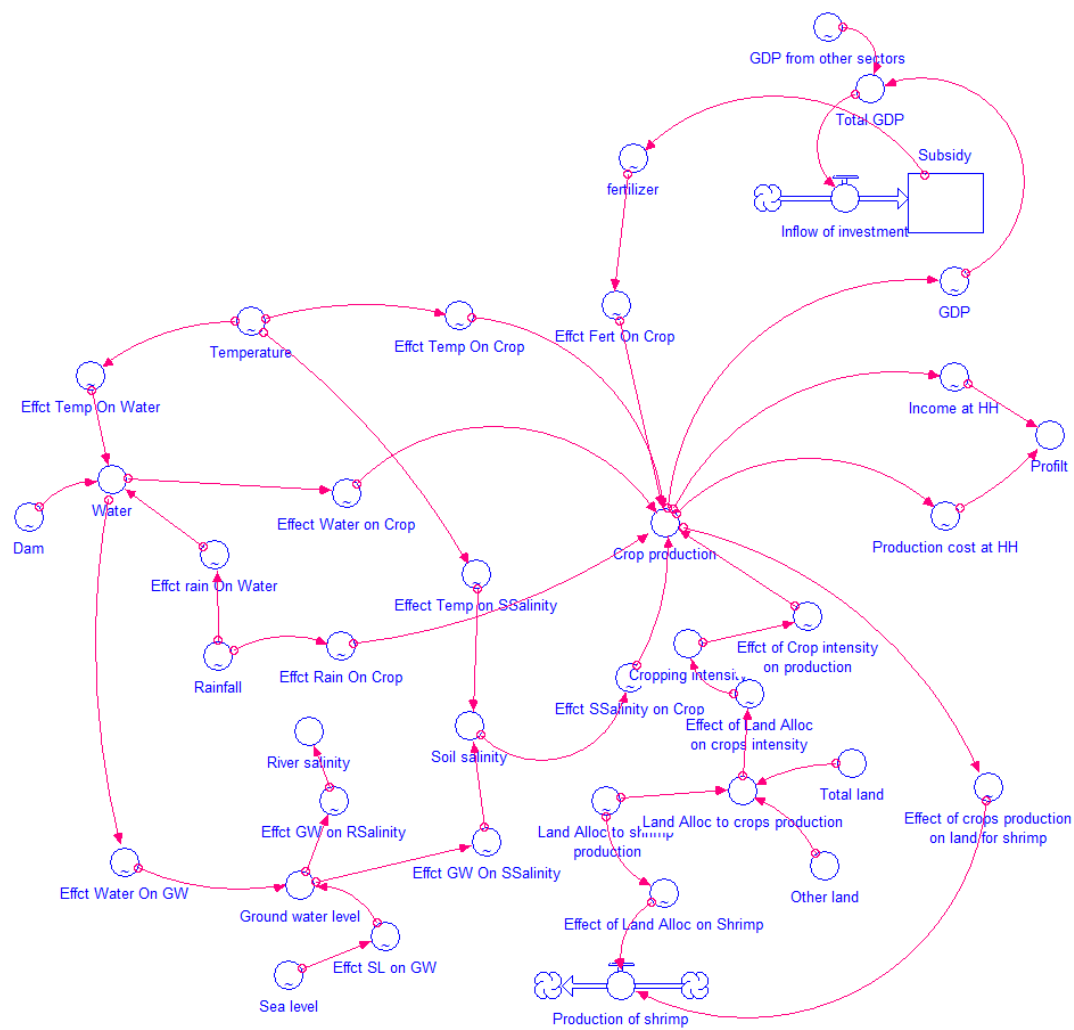
SI Figure 5 Full system dynamic model in STELLA depicting the converters, stock, flow and connections detailed in SI equation 1
