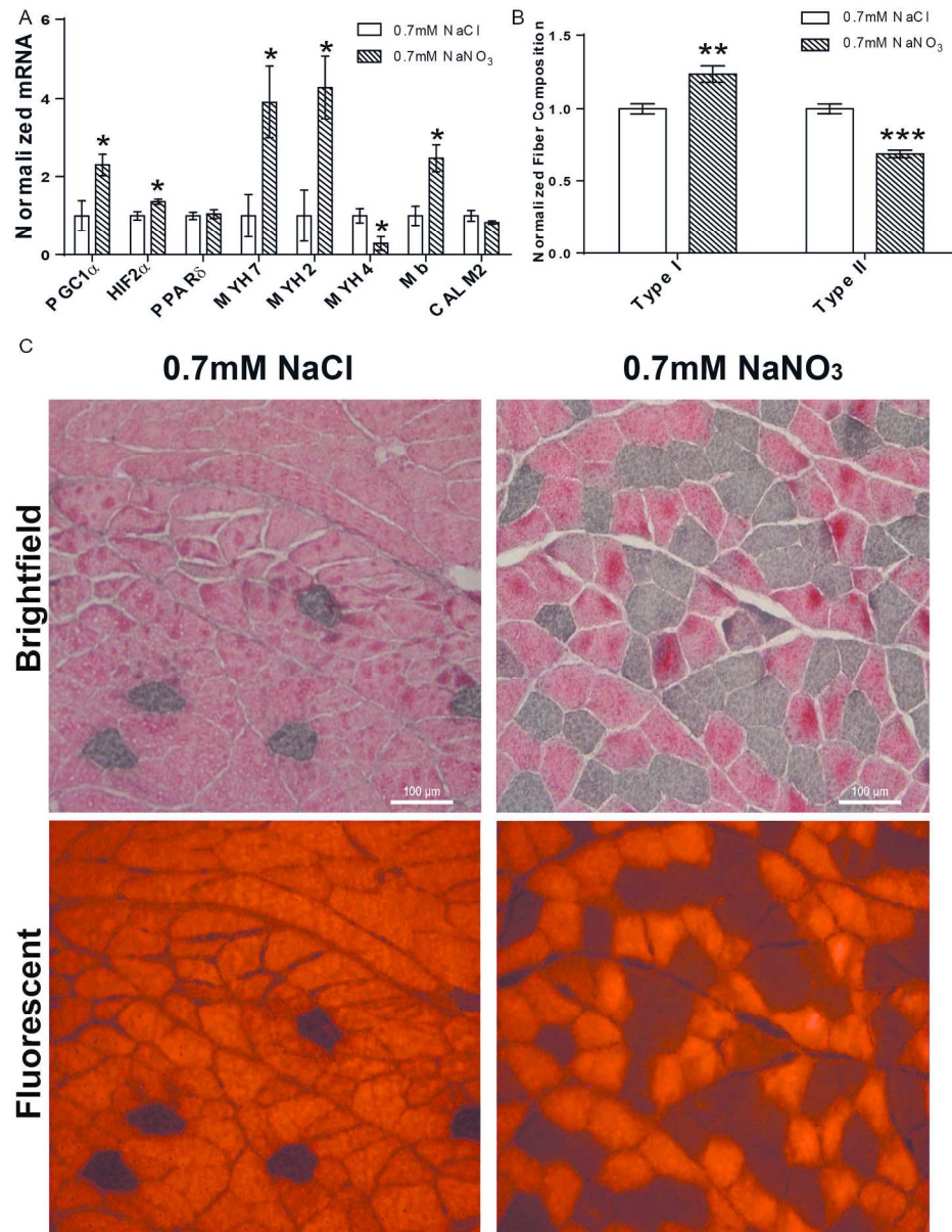
Fig 2. Inorganic Nitrate Induces Muscular Fiber-type Switching in Glycolytic Muscle (A) The expression of slow and intermediate-twitch muscle fiber genes, PGC1 \alpha , HIF2 \alpha , MYH7, MYH2 and Mb, and the fast-twitch muscle fiber gene MYH4 in nitrate treated rat gastrocnemius (multiple t-test, n = 4 ). (B) Quantitation of fiber-types from cross-sections of gastrocnemius immunostained for myosin heavy chains I and II ( n = 4 ). (C) Cross-sections of gastrocnemius were immunostained for myosin heavy chains I (black/grey), II (red) (fluorescent red) ( n = 4 ). Original magnification, \times 20 . Data are represented as Mean \pm SEM. *, P \leq 0.05 , **, P \leq 0.01 , *** P \leq 0.001 .
