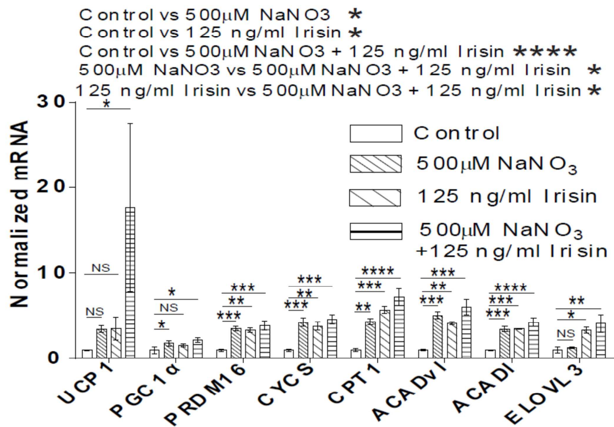
Fig S3. The effect of nitrate and irisin on brown adipocyte-specific gene expression is additive. Expression of brown adipocyte-associated genes in primary adipocytes treated with 500 μM NaNO 3 with and without 125 ng/ml irisin (one-way ANOVA, n = 3). Uncoupling protein 1 (UCP1), peroxisome proliferator-activated receptor γ coactivator 1α (PGC1α), PR domain containing 16 (PRDM16), cytochrome C (CYCS), carnitine palmitoyltransferase 1 (CPT1), acyl-CoA dehydrogenases, very long chain (ACADvl) and long chain (ACADI) and fatty acid elongase 3 (ELOVL3). Results of two-way ANOVA omnibus test are shown at the top of the graph. Data are represented as Mean ± SEM. * P ≤ 0.05, ** P ≤ 0.01, *** P ≤ 0.001, **** P < 0.0001.
