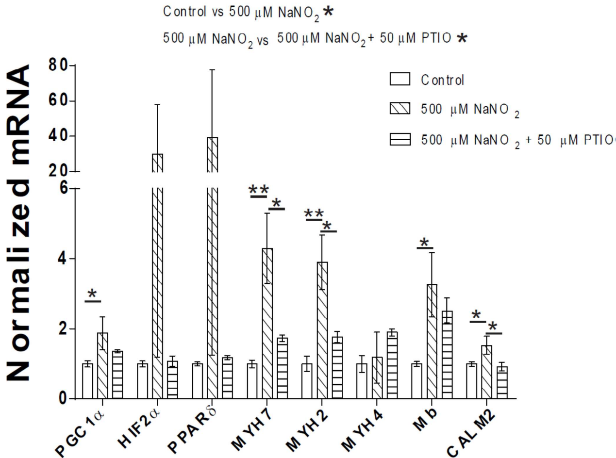
Fig S1. The nitrite-mediated expression of oxidative muscle fiber-type associated genes is abrogated by nitric oxide sequestration. The expression of slow, intermediate and fast-twitch muscle fiber genes peroxisome proliferator-activated receptor \gamma coactivator 1 \alpha (PGC1 \alpha ), hypoxia-inducible factor 2 \alpha (HIF2 \alpha ), peroxisome proliferator activated receptor \delta (PPAR \delta ), myosin heavy chain 7 (MYH7), myosin heavy chain 2 (MYH2), calmodulin 2 (CALM2), and myosin heavy chain 4 (MYH4) in C2C12 myotubes treated with nitrite (500 \mu\text{M} \text{NaNO}_2 ), and nitrite and PTIO (500 \mu\text{M} \text{NaNO}_2 + 50 \mu\text{M} PTIO) (one-way ANOVA, n = 3). Results of two-way ANOVA omnibus test are shown at the top of the graph. *, P \leq 0.05 , **, P \leq 0.01 .
