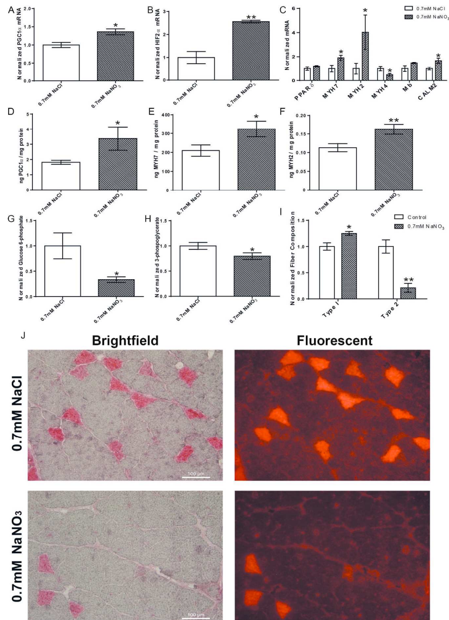
Fig 1. Inorganic Nitrate Induces Muscular Fiber-type Switching in Oxidative Muscle (A) PGC1α mRNA in nitrate treated rat soleus (t-test, n = 5). (B) HIF2α mRNA in nitrate treated rat soleus (t-test, n = 5). (C) The expression of slow and intermediate-twitch muscle fiber genes, MYH7, MYH2, CALM2, and the fast-twitch fiber gene, MYH4, in nitrate treated rat soleus (multiple t-test, n = 5). (D) PGC1α protein in nitrate treated rat soleus (t-test, n = 5 / group). (E) MYH7 protein concentration in nitrate treated rat soleus (t-test, n = 5). (F) MYH2 protein concentration in nitrate treated rat soleus (t-test, n = 5). (G) Glucose-6-phosphate concentration in nitrate treated rat soleus (t-test, n = 9). (H) 3-phosphoglycerate concentration in nitrate treated rat soleus (t-test, n = 9). (I) Quantitation of fiber-types from cross-sections of soleus immunostained for myosin heavy chains I and II (n = 5). (J) Cross-sections of soleus immunostained for myosin heavy chains I (black/grey), II (red) (fluorescent red) (n = 5) Original magnification, × 20. Data are represented as Mean ± SEM. *, P ≤ 0.05, **, P ≤ 0.01.
