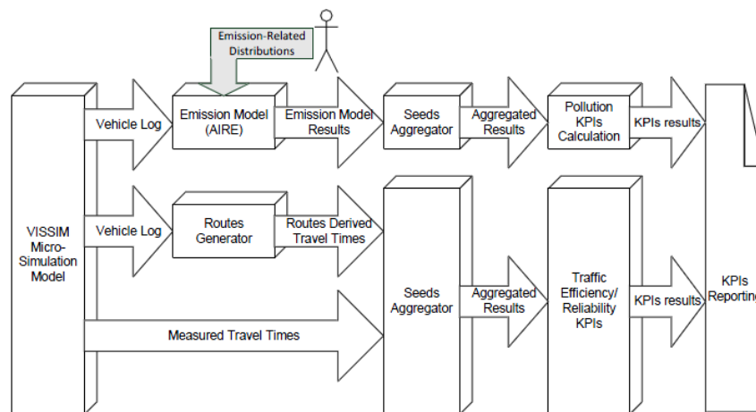
FIGURE 1: CONDUITS_DST structure and components [6]
