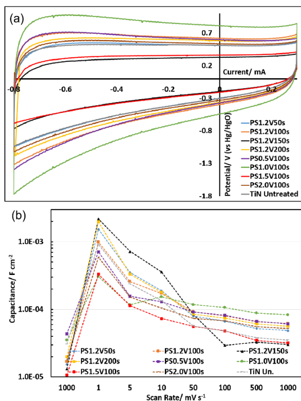
Fig. 5 (a) Cyclic voltammograms in 6 mol dm -3 KOH (50 th cycle of the final set at 1000 mV s -1 ) in 6 mol dm -3 KOH of the of as-prepared and potential step oxidised TiN, and (b) areal specific capacitance values at the middle cycle of each of the sequential scan rates of PSO1.2V50s, PSO1.2V100s, PSO1.2V150s and PSO1.2V200s were oxidised at 1.2 V for 50 s, 100 s, 150 s and 200 s respectively and PSO0.5V100s, PSO1.0V100s, PSO1.5V100s and PSO2.0V100s were oxidised for 100 s at 0.5 V, 1.0 V, 1.5 V and 2.0 V respectively.
