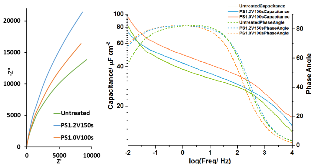
Fig. 7 Nyquist plot of the EIS (left) and areal capacitance vs frequency plot (right) of untreated TiN, PS1.2V150s and PS1.0V100s electrodes collected at the open circuit potential (~-0.4 V).
