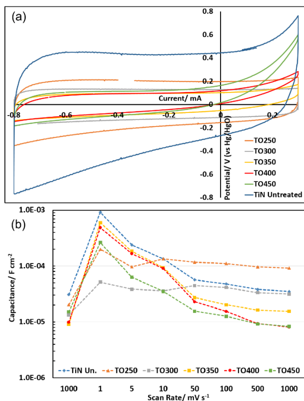
Fig. 4 (a) Cyclic voltammograms in 6 \text{ mol dm}^{-3} KOH (5 th cycle at 1000 \text{ mV s}^{-1} ) of as-prepared and thermally oxidised TiN samples, and (b) areal specific capacitance values at the 5 th cycle at each of the sequential scan rates. TO250, TO300, TO350, TO400 and TO450 represent oxidation at 250, 300, 350, 400 and 450^\circ\text{C} respectively.
