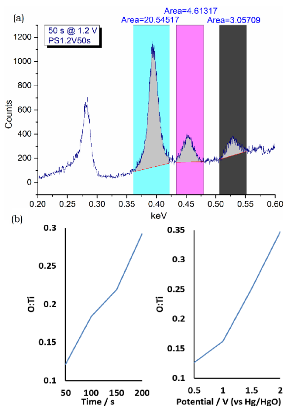
Fig. 8 (a) Exemplar integrated WDX spectrum of a potential step oxidised TiN foil showing the regions used to analyse Ti+N, Ti and O content (top, full set of spectra in Figs. S22-S24), (b) and the calculated O:Ti ratios compared with time at 1.2 V (bottom left) and potential at 100 s (bottom right).
