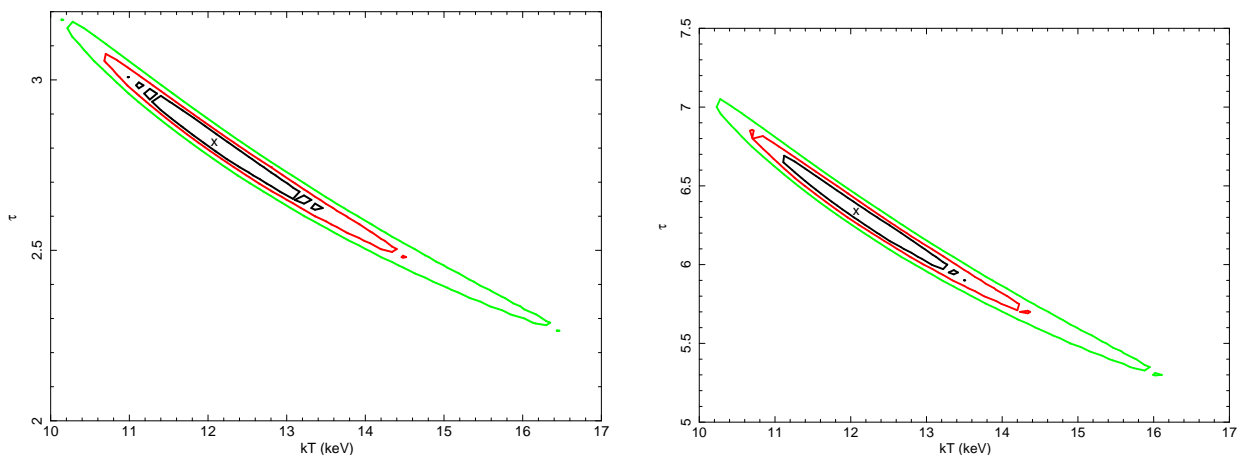
Figure 8. Coronal temperature vs optical depth contour plot in the case of slab geometry (left panel) and spherical geometry (right panel) for the NuSTAR observation when the COMPIT model is used to fit the data. The solid black, red and green curves refer to the 68, 90 and 99% confidence levels respectively. The X represents the best fit value of the parameters.
