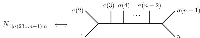
Figure 2. Master diagrams with respect to Jacobi relations which are associated with the master numerators N_{1|\sigma(23\dots n-1)|n} defined by (5.3).
