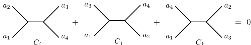
Figure 1. The Jacobi identity f^{a_1 a_2 b} f^{b a_3 a_4} + \text{cyc}(a_1, a_2, a_3) implies the vanishing of the color factors C_i , C_j and C_k associated to triplets of cubic graphs. In the above diagrams, the legs a_1, \dots, a_4 may represent arbitrary cubic tree-level subdiagrams. The duality between color and kinematics states that their corresponding kinematic numerators N_i built from polynomials of Mandelstam invariant for the cases of interest can be chosen such that N_i + N_j + N_k = 0 whenever C_i + C_j + C_k = 0 [5].
