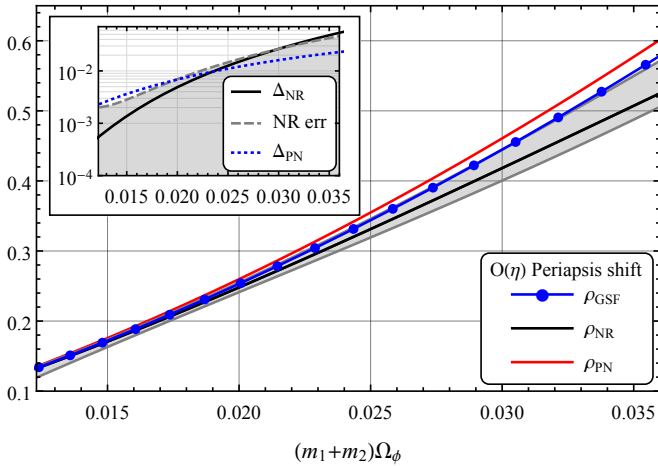
Figure 1. Comparison of our (exact) numerical calculation of the linear in mass ratio correction to the periaapsis advance, \rho_{\text{GSF}} , to previous NR \rho_{\text{NR}} and PN \rho_{\text{PN}} estimates at a = -0.5 provided in [32]. The inset shows the differences \Delta_{\text{NR}} = |\rho_{\text{NR}} - \rho_{\text{GSF}}| and \Delta_{\text{PN}} = |\rho_{\text{PN}} - \rho_{\text{GSF}}| on a semi-Log-scale. The shade region indicates the error on the NR estimate.
