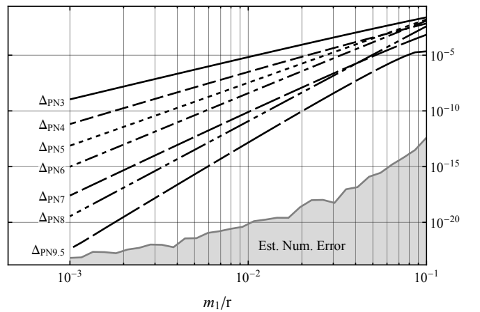
Figure 2. Log-Log plot of the residual differences \Delta_{\text{PN}n} := |\rho_{\text{GSF}} - \rho_{\text{PN}n}| between our calculation of \rho_{\text{GSF}} at a = 0 and successive PN approximants \rho_{\text{PN}n} provided in [34]. The shaded area indicates the estimated numerical error on the self-force result.
