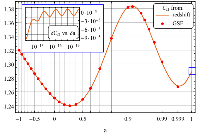
Figure 3. Comparison of two methods for calculating the ISCO shift from either GSF or redshift data. The x-axis has had a non-linear scaling applied to better display the new phenomenology in the a > 0.9 region. The inset shows a close-up of the near extremal limit plotting \delta C = C_\Omega - C_1 vs. \delta a = 1 - a , revealing persistent order 10^{-5} oscillations.
