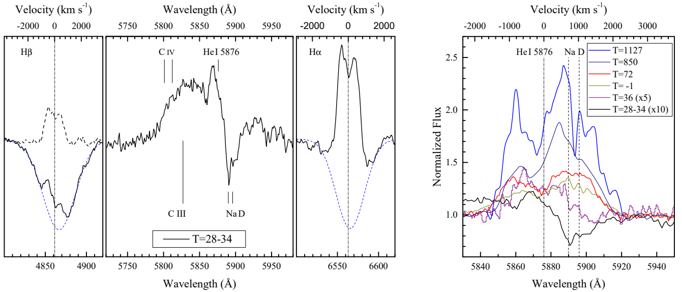
Figure 14. Left: H\alpha and H\beta line profiles and the region around the C III / C IV / He I \lambda 5876 / Na D complex (black solid line) during the plateau stage of the superoutburst (arbitrary scaling). The dashed blue line shows a Gaussian fit to the absorption components of H\alpha and H\beta . The dashed black line shows the profile of H\beta after being corrected for absorption. Right: He I \lambda 5876 and Na D line profiles from different data sets, shown in actual scale (for a better comparison, the T=28 – 34 and 36 profiles have been multiplied by a factor of 10 and 5, respectively).
