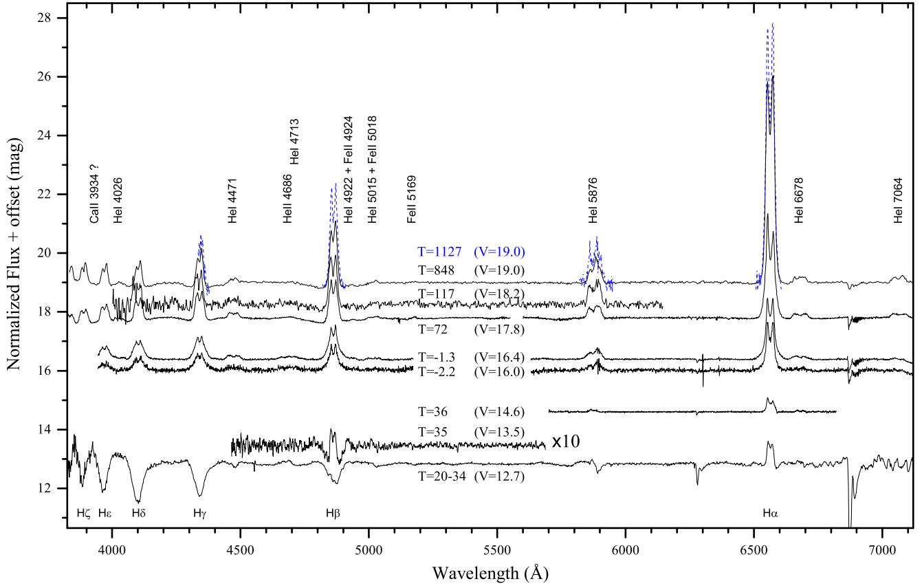
Figure 13. Spectral evolution of SSS J122221 through all the outburst stages and the following decay. All the spectra are normalized to the continuum flux and shifted with respect to each other in accordance to the magnitude of the system during the given spectral observation. Thus, the outburst spectra ( V \approx 12.7 ) are at the bottom and the quiescent spectra ( V \approx 18 – 19 ) are at the top of the figure. The T=1127 spectrum is relatively noisy at the continuum level, therefore we only show the emission lines (a dashed blue line). Two lower outburst spectra are scaled up by a factor of 10 in relative intensity to magnify the spectral features and allow for a better comparison.
