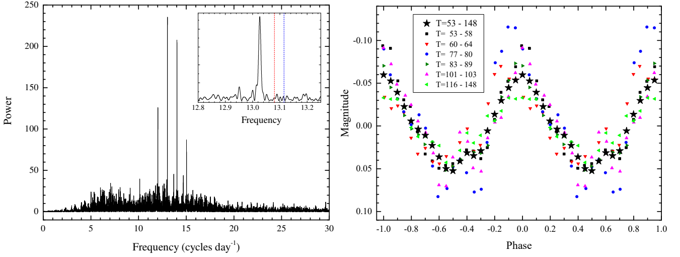
Figure 10. Left: Lomb–Scargle periodogram of the V data combined between T=53 and 148. The inset shows the enlarged region around the frequency 13.026 cycle d -1 – the frequency of post-superoutburst modulations observed in 2013. The vertical dashed lines mark the orbital (blue) and stage B superhump (red) frequencies of 13.11 and 13.08 cycle d -1 , respectively. Right: the entire set (large stars) and short subsets (small symbols) of the V data between T=53 and 148, folded according to ephemeris HJD_{max} = 245\,6300.0610(3) + 0.07676887(5) \cdot E .
