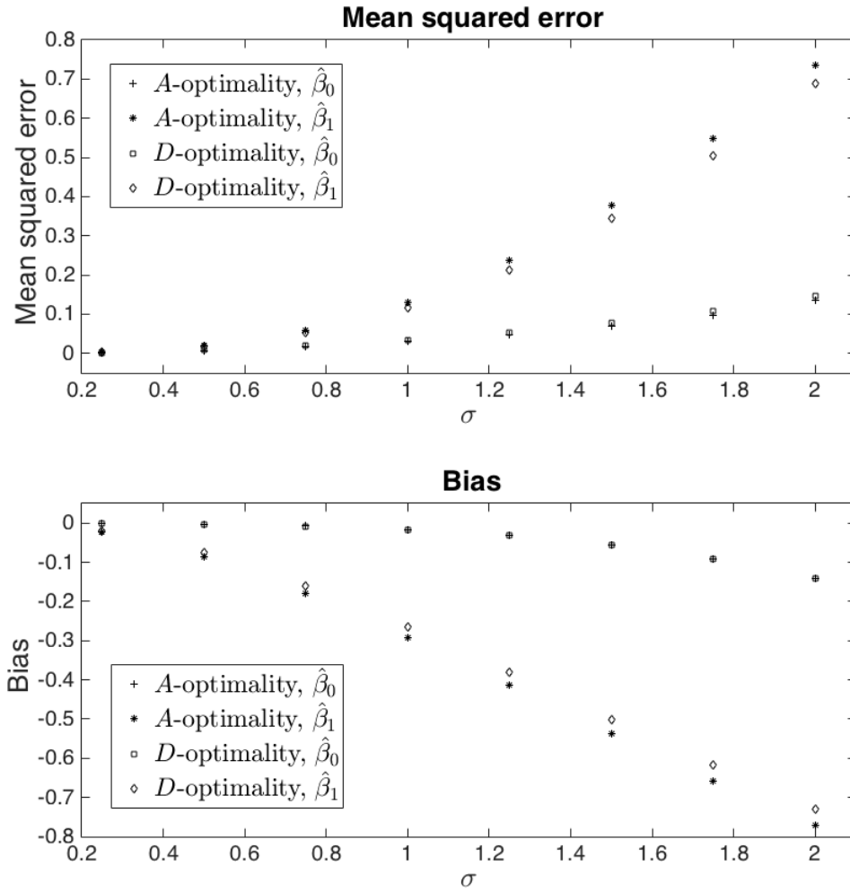
Figure 1: Mean squared error and bias of the estimates that are computed using the A - and the D -optimal design in the presence of NMAR mechanisms.
