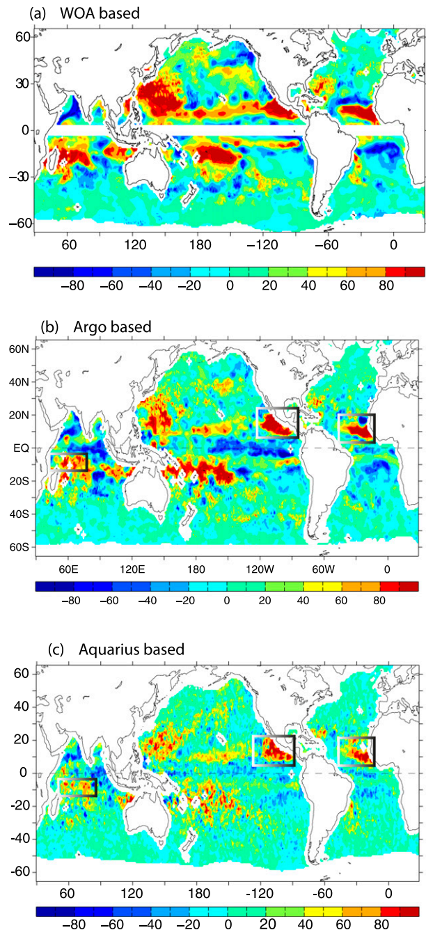
FIG. 13. The percentage of seasonal variances of surface salinity that can be explained by E - P from OAFlux-GPCP based on (a) WOA MLS, (b) Argo MLS, and (c) Aquarius SSS. The three boxed areas are chosen as the test sites for using salinity to assess the uncertainty in E - P products.
