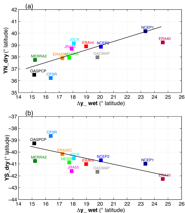
FIG. 6. The width of the tropical wet zone ( x axis) vs the latitudinal position of the poleward edge of the subtropical dry zone ( y axis) in the (a) Northern Hemisphere and (b) Southern Hemisphere.
