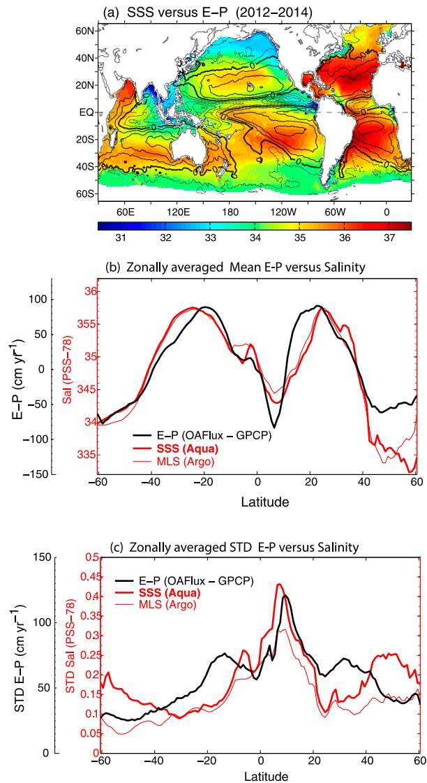
FIG. 12. (a) Mean Aquarius SSS with the E - P contours (black) of the same three years superimposed. (b) Zonal mean average of Aquarius SSS (thick red), Argo MLS (thin red), and E - P from OAFlux-GPCP (black). (c) Zonal average of seasonal STD of Aquarius SSS (thick red), Argo MLS (thin red), and E - P from OAFlux-GPCP (black). All fields are based on the 3-yr climatology of 2012–14.
