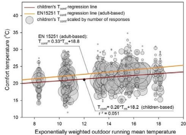
Fig. 1. Relationship between the children’s comfort temperature and the running mean of the outdoor temperature with regression line. The line used in the European standard EN 15251 is also included for comparison.
