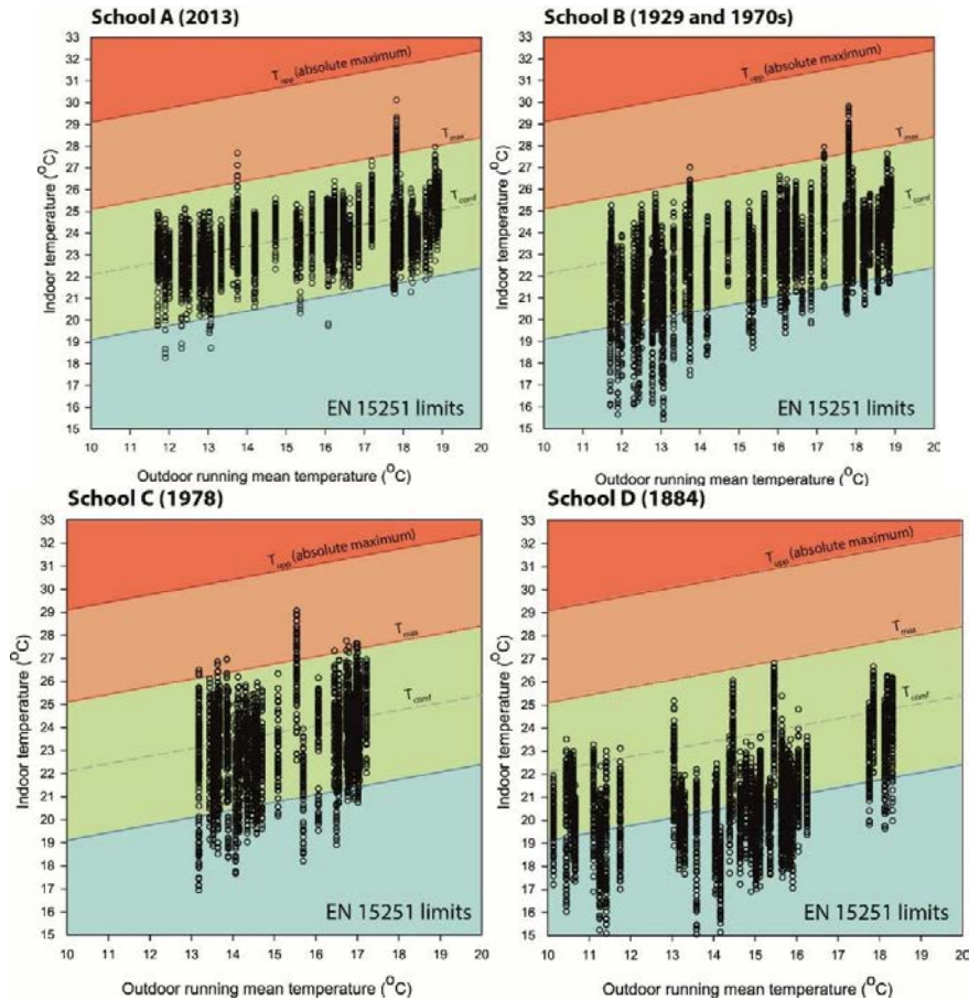
Fig. 2. Measured hourly air temperatures during occupied hours in each school against the outdoor running mean temperature. The EN 15251 temperature limits used for the overheating assessment are also illustrated.
