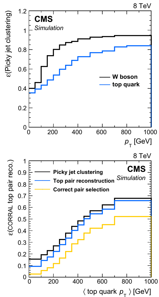
Fig. 2 Efficiency as a function of generator level p_T for picky jet clustering and CORRAL top quark pair reconstruction in all-hadronic T2tt events with m_{\tilde{\chi}_1^0} = 600 GeV and m_{\tilde{\chi}_1^\pm} = 50 GeV. Top The efficiency to correctly cluster final state particles from each W boson and top quark decay into two and three picky jets, respectively, as a function of particle (top quark or W boson) p_T . Bottom The efficiency at each stage of the CORRAL algorithm to reconstruct a hadronically decaying top quark pair as a function of the average p_T of the two top quarks. They are the efficiency to correctly cluster the final state particles from top quark decays into six picky jets, labelled “Picky jet clustering”; the efficiency to both carry out picky jet clustering and reconstruct the top quark pair with these six picky jets, labelled “Top pair reconstruction”; and finally the efficiency to carry out picky jet clustering, top pair reconstruction, and then correctly select the reconstructed top quark pair for use in the analysis, labelled “Correct pair selection”
