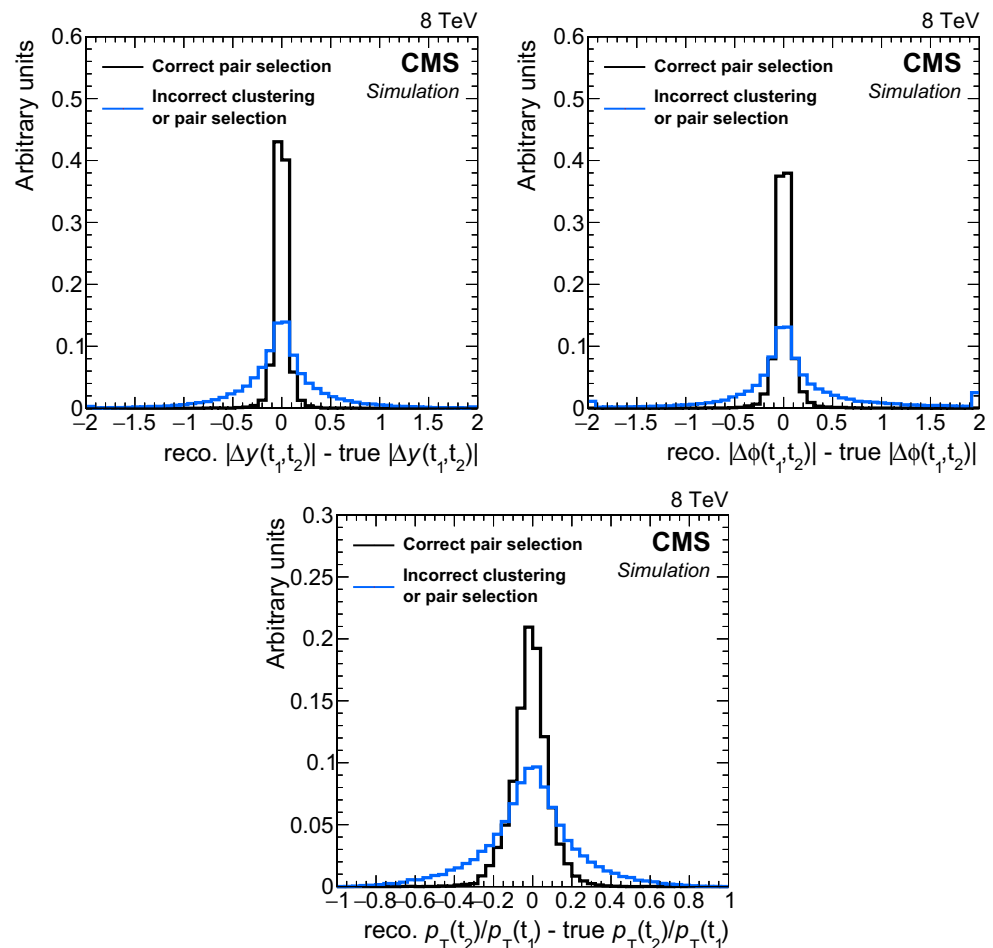
Fig. 4 Properties of the reconstructed top quark pair used in the analysis are compared to their true properties in all-hadronic T2tt events with m_{\tilde{t}} = 600 GeV and m_{\tilde{\chi}_1^0} = 50 GeV. The label “Correct pair selection” corresponds to events in which the two top quark decays are each resolved into three distinct picky jets and these jets are used to reconstruct the two top quarks. The label “Incorrect clustering or pair selection” is used for all other events. The top two figures show comparisons of the angular separation between the two top quarks in rapidity, y \equiv -(1/2) \ln[(E + p_z)/(E - p_z)] , and azimuthal angle \phi . The bottom figure compares the relative p_T of the two top quarks. In all cases, t_1 refers to the top quark with the highest p_T
