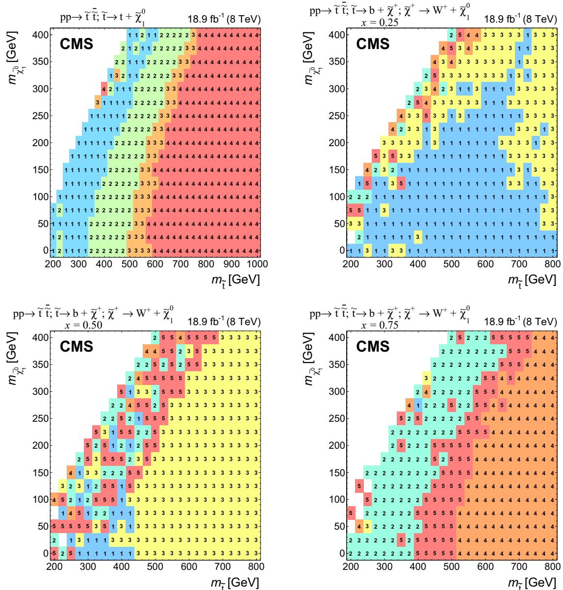
Fig. 7 Search regions providing the most stringent limits in the m_T - m_{\tilde{\chi}_1^0} plane in the T2tt signal topology ( top left ) and the T2bW signal topologies for mass splitting parameter values x = 0.25, 0.50, 0.75 . The T2tt_LM, T2tt_MM, T2tt_HM, and T2tt_VHM search regions are numbered 1, 2, 3, and 4, respectively. The T2bW_LX, T2bW_LM,
