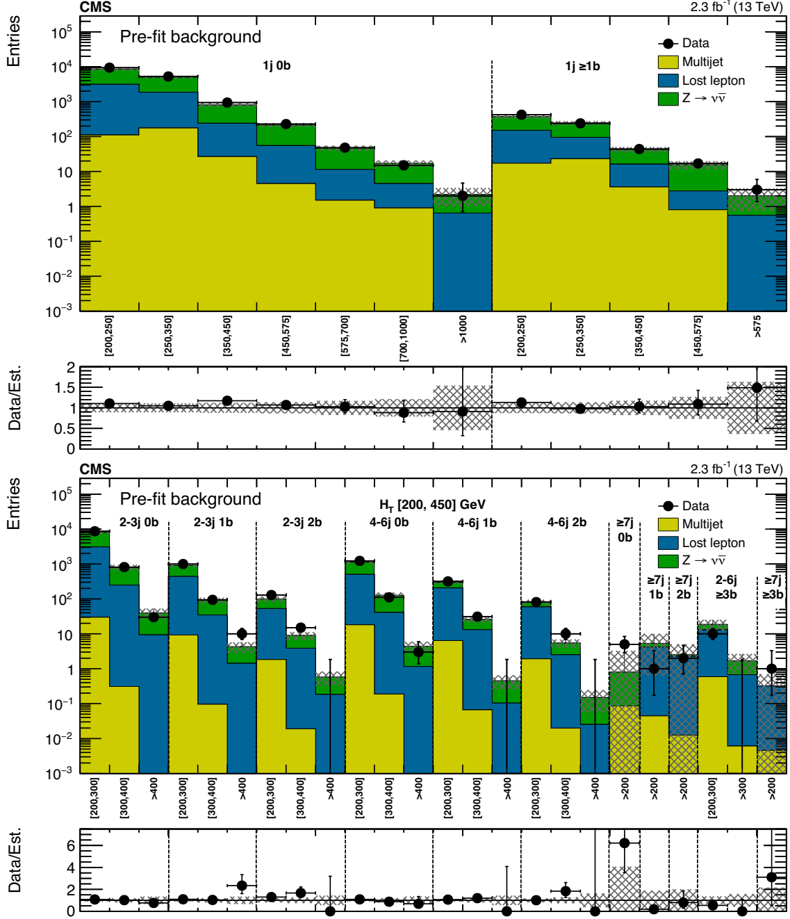
Figure 12. (Above) Comparison of the estimated background (pre-fit) and observed data events in each signal bin in the monojet region. On the x -axis, the jet p_T binning is shown (in GeV). Hatched bands represent the full uncertainty in the background estimate. (Below) Same for the very-low- H_T region. On the x -axis, the M_{T2} binning is shown (in GeV). Bins with no entry for data have an observed count of 0 events.
