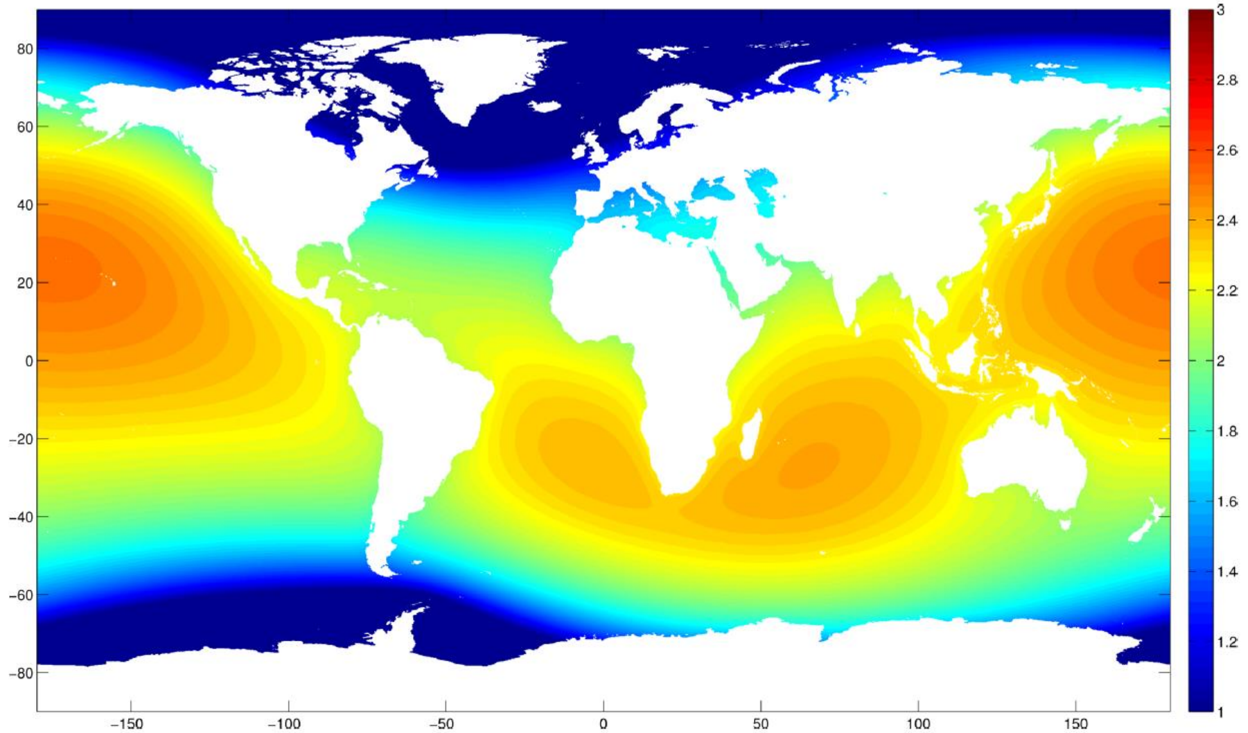
Fig. 5. The SLR perturbation (m) applied to the model for the 2m average SLR non-uniform initial elastic response scenario with uniform ice sheet melt in both Greenland (1m) and Western Antarctica (1m) (+2NUB). In the near field of the areas of the mass loss sea-level change can be negative. For coastal city SLR values see Table SM1. Data courtesy of Mitrovica et al. (2001).
