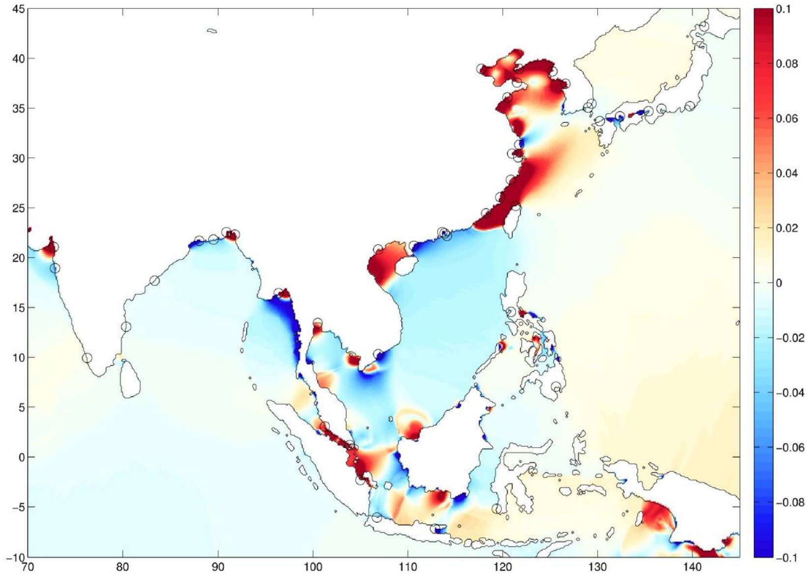
Fig. 3. Asian change in MHW (m) with 2m of uniform SLR assuming a fixed present day coastline (+2UF) (increases- red, decreases- blue). For coastal city changes, marked by the black circles, see Tables 4 and 5. (Regional zoom of Fig. 2a)
