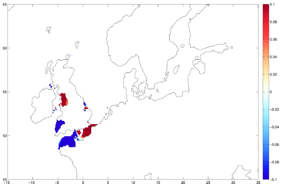
Fig. 7. European change in maximum range (m), over the 15 day SSH reconstruction based on the four tidal constituents, with a 2m uniform SLR assuming a fixed coastline (+2UF) (increases- red, decreases- blue) for those locations found to be presently viable for tidal renewable energy (either 25-100m depth and peak current velocities >2m/s or with a MTR > 5m).
