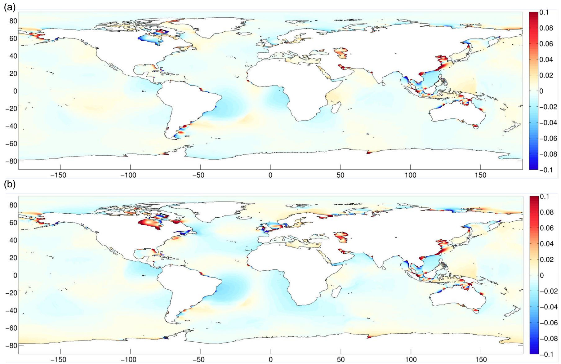
Fig. 6a. Change in MHW (m) with an average of 2m of non-uniform SLR from (a) Greenland (Fig. SM17) assuming a fixed coastline (+2NUGF) (b) Western Antarctica (Fig. SM18) assuming a fixed coastline (+2NUWAF) (increases- red, decreases- blue). For coastal city changes see Table 8.
