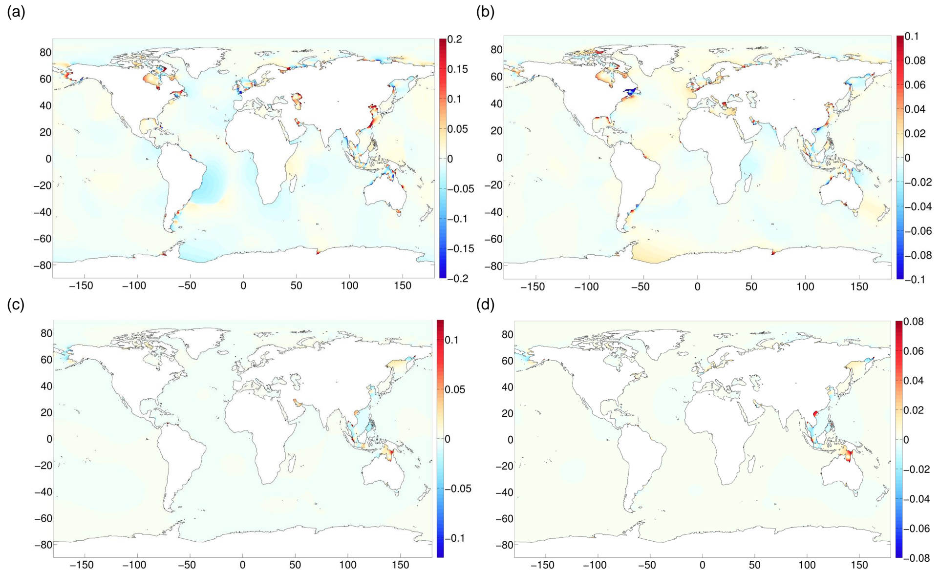
Figs. 1a-d. Change in amplitude (m) of M2 (a), S2 (b), K1(c) and O1 (d) with 2m of uniform SLR assuming a fixed present day coastline (+2UF) (increases- red, decreases- blue). Colour scale limits between constituents scaled in proportion to equilibrium tidal amplitudes. For coastal city changes see Table 4. 17
