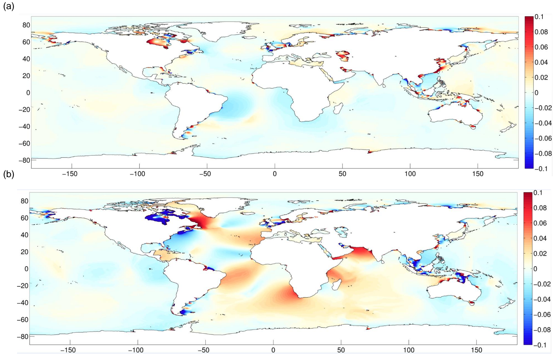
Fig. 2. (a) Change in MHW (m) with 2m of uniform SLR assuming a fixed present day coastline (+2UF) (increases- red, decreases- blue). For coastal city changes see Table 4 and 5. (b) Change in MHW (m) with 2m of uniform SLR permitting coastal recession (+2UR), except around Antarctica (increases- red, decreases- blue). For coastal city changes see Table 4. For newly wet areas in the SLR scenario the now calculable MHW values are plotted on the positive part of the colour scale.
