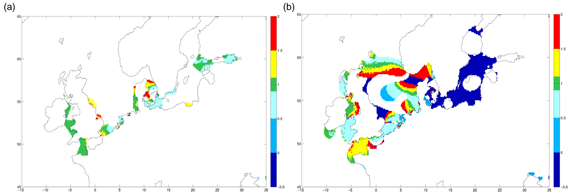
Fig. 4. European normalised proportionality ratio of the significant MHW change with (a) 1m uniform SLR (+1UF) and (b) 5m uniform SLR (+5UF) to the MHW change with 0.5m uniform SLR (+0.5UF) assuming a fixed coastline. Proportional change is given by a ratio of 1 (+/- 0.1). Ratio values <0.9 (>1.1) or <0 show a below (above) proportional change or sign change of the MHW response in the SLR scenario. Insignificant MHW Changes (<+/- >- 5cm) are masked out. Black circles mark coastal cities.
