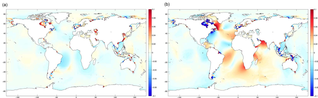
Fig. 2. (a) Change in MHW (m) with 2 m of uniform SLR assuming a fixed present day coastline (+2UF) (increases- red, decreases- blue). For coastal city changes see Tables 4, 5. (b) Change in MHW (m) with 2 m of uniform SLR permitting coastal recession (+2UR), except around Antarctica (increases- red, decreases- blue). For coastal city changes see Table 4. For newly wet areas in the SLR scenario the now calculable MHW values are plotted on the positive part of the colour scale.
