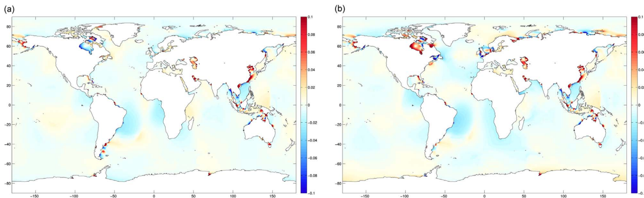
Fig. 6. a. Change in MHW (m) with an average of 2 m of non-uniform SLR from (a) Greenland (Fig. SM17) assuming a fixed coastline (+2NUGF) (b) Western Antarctica (Fig. SM18) assuming a fixed coastline (+2NUWAF) (increases- red, decreases- blue). For coastal city changes see Table 8.
