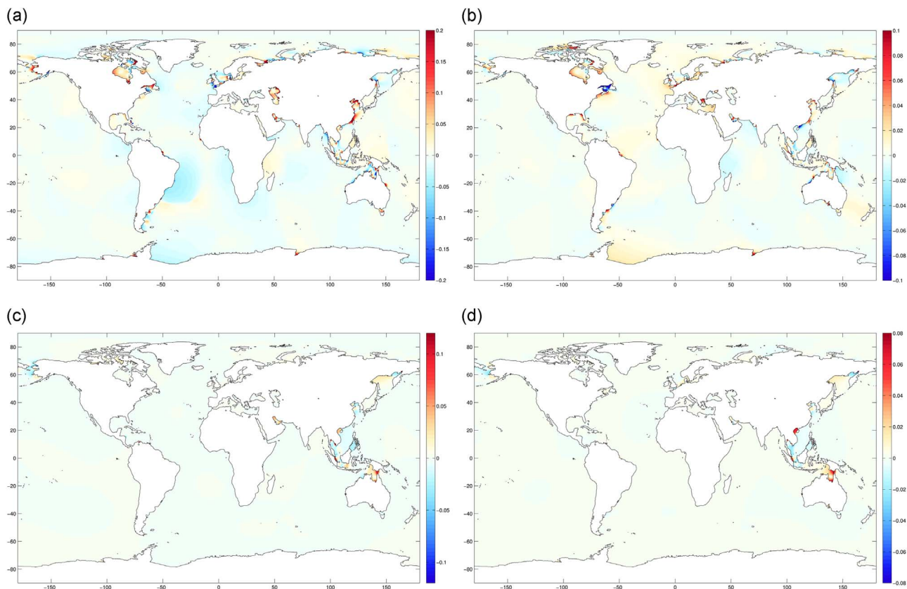
Fig. 1. a-d. Change in amplitude (m) of M2 (a), S2 (b), K1(c) and O1 (d) with 2 m of uniform SLR assuming a fixed present day coastline (+2UF) (increases- red, decreases- blue). Colour scale limits between constituents scaled in proportion to equilibrium tidal amplitudes. For coastal city changes see Table 4.
