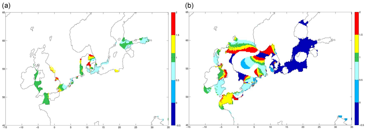
Fig. 4. a. European normalised proportionality ratio of the significant MHW change with (a) 1 m uniform SLR (+1UF) and (b) 5 m uniform SLR (+5UF) to the MHW change with 0.5 m uniform SLR (+0.5UF) assuming a fixed coastline. Proportional change is given by a ratio of 1 (+/- 0.1). Ratio values < 0.9 ( > 1.1 ) or < 0 ( > 1 ) show a below (above) proportional change or sign change of the MHW response in the SLR scenario. Insignificant MHW Changes ( < +/- > 5 cm) are masked out. Black circles mark coastal cities.
