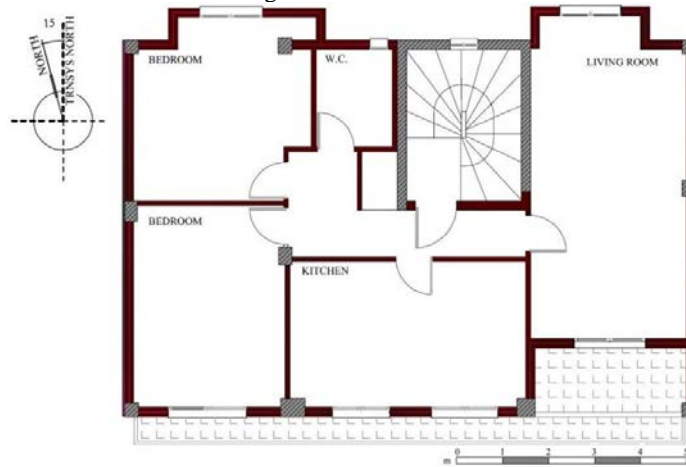
Fig. 1. Floor plan of the case study building Brick masonry walls are indicated in red and load bearing frame in grey.
