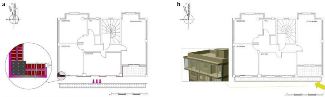
Fig. 3. (a) The South façade intervention, showing the dismissed balcony part and a close view of the corner intercept with the previously refurbished West façade; (b) Illustration of the proposed solution on the 3rd floor
