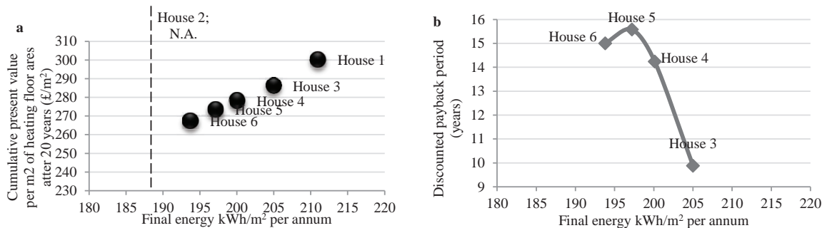
Fig. 6. (a) Cumulative present value of the overall investment and energy costs over a 20-year timeframe; (b) Discounted payback period (House 1: Current, House 2: Coldbridge_free, House 3:ThB_insulation, House 4:Ext_insulation, House 5: Demolition, House 6: Sunspace)
