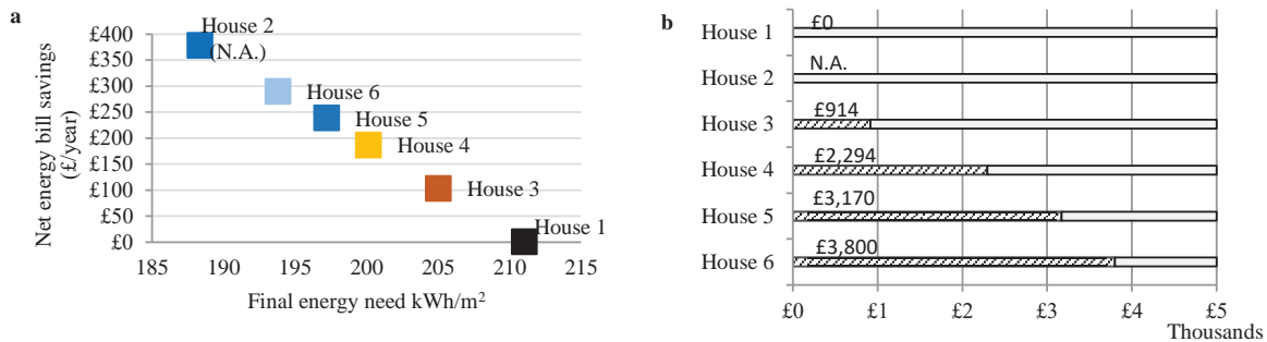
Fig. 5. (a) Net energy savings per year for each of the solutions; (b) Total cost of intervention for each of the solutions. (House 1: Current, House 2: Coldbridge_free non-applicable, House 3: ThB_insulation, House 4: Ext_insulation, House 5: Demolition, House 6: Sunspace)
