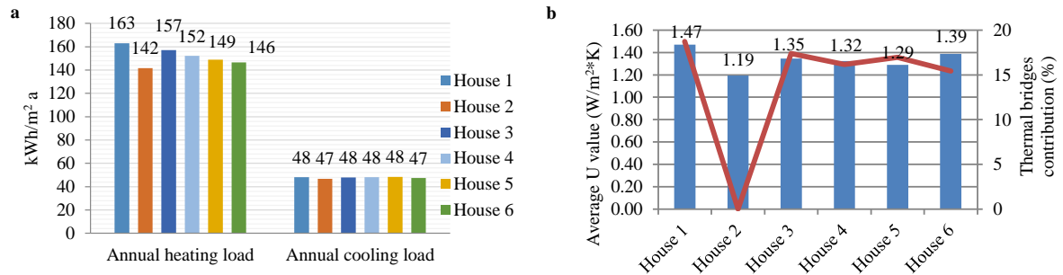
Fig. 4. (a) Annual heating and cooling loads for all the models ( \text{kWh/m}^2 per annum); (b) Average U value (thermal bridges included) of the all the models (House 1-6) and percentage of thermal bridges on the total heat loss through the fabric elements. (House 1: Current, House 2: Coldbridge_free, House 3: ThB_insulation, House 4: Ext_insulation, House 5: Demolition, House 6: Sunspace)
