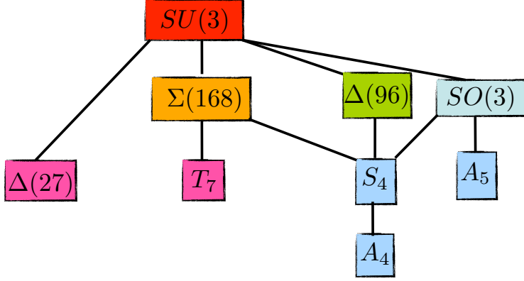
Figure 12: Some popular family symmetries and their relationships.
