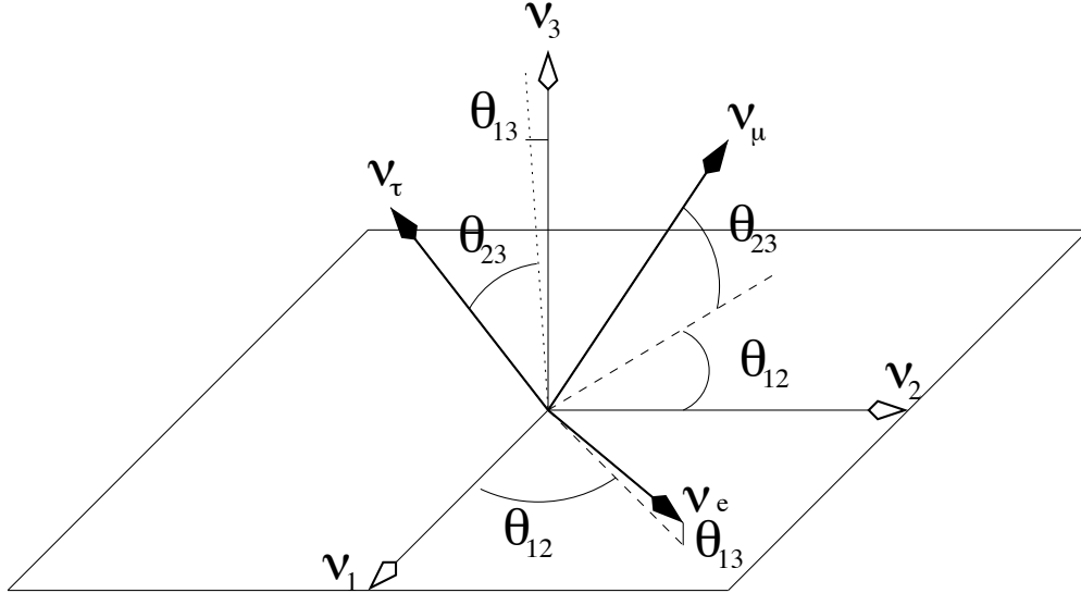
Figure 1: Neutrino mixing angles (assuming zero \mathcal{CP} violation) may be represented as Euler angles relating the charged lepton mass basis states (\nu_e, \nu_\mu, \nu_\tau) to the mass eigenstate basis states (\nu_1, \nu_2, \nu_3) .
