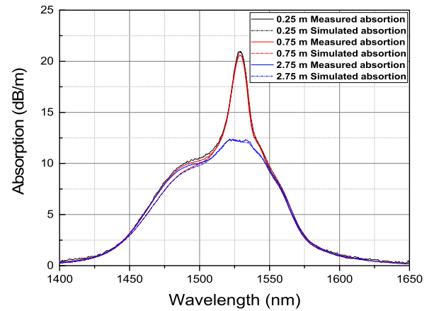
Fig. 5. Apparent absorption spectra per unit length determined with WLS & OSA for three different EDF cutback lengths with NA = 0.242. The experimental and simulated curves agree very well and are difficult to distinguish. In addition, the curves for 0.25 m and 0.75 m are quite close and also difficult to distinguish.
