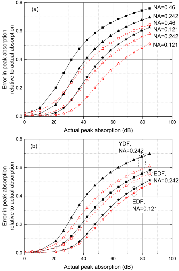
Fig. 10. (a) Error in peak absorption measured with TLS and broadband detection relative to actual peak absorption ((\alpha - \alpha_{TLS}) / \alpha) for EDFs (red dotted curves with empty data markers) and YDFs (black solid curves with filled data markers) of different NA with V = 2 . (b) Selected curves from (a) (black solid curves with filled data markers) together with matching curves from Fig. 8 for WLS and OSA (red dotted curves with empty data markers).
