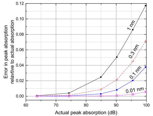
Fig. 12. Simulation of the relative measurement error ((\alpha - \alpha_{WLS}) / \alpha) at the absorption peak for different largest value of source and detector bandwidth for EDF with NA of 0.242.
