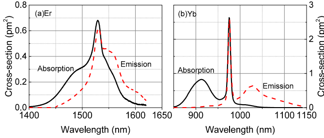
Fig. 3. Cross-section spectra used in simulations, (a) Er:aluminosilicate, (b) Yb:germanosilicate. From [11], [12].
