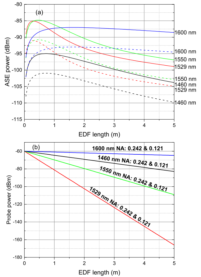
Fig. 7. Evolution of power within 1 nm along EDFs with NA 0.242 and 0.121 at different wavelengths, (a) fluorescence power (NA = 0.242: solid curve; NA = 0.121: dashed curve), (b) probe power. Note difference in power axis scales.
