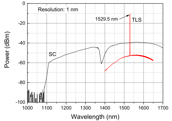
Fig. 2. Spectrum of SC-source and TLS as launched into the EDF.
