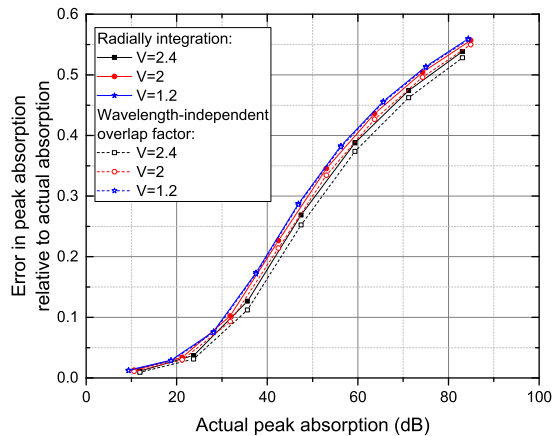
Fig. 14. Error in absorption relative to actual absorption ( (\alpha - \alpha_{WLS}) / \alpha ) at absorption peak with the WLS + OSA configuration for an 0.242-NA EDF of three different V-values obtained with radially resolved simulations (solid curves) and with wavelength-independent overlap factors (dotted curves).
