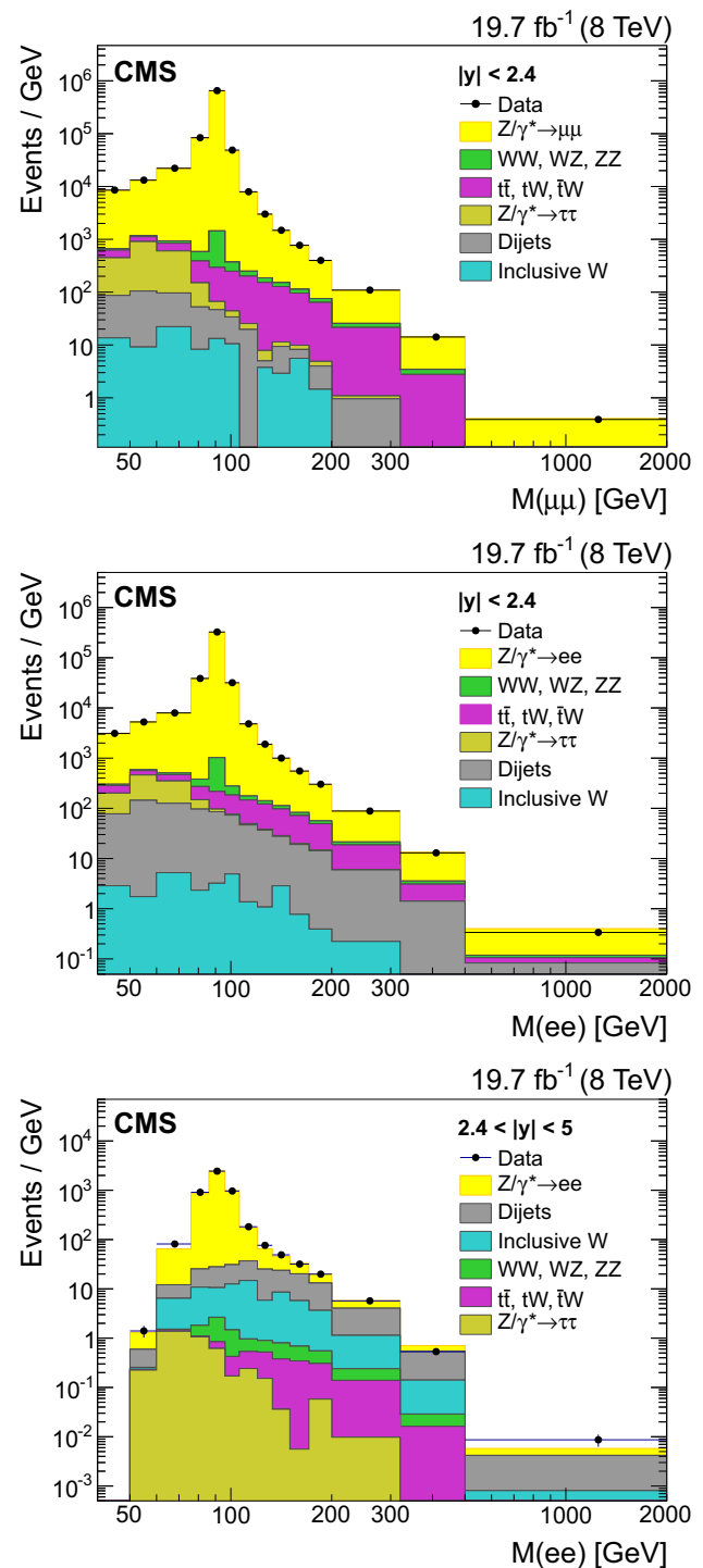
Fig. 1 The invariant mass distributions for \mu\mu (top), ee (middle) events with |\gamma| < 2.4 , and ee (bottom) events with 2.4 < |\gamma| < 5 . Only statistical uncertainties are shown. The stacked histograms represent the sum of the background contributions and the signal
