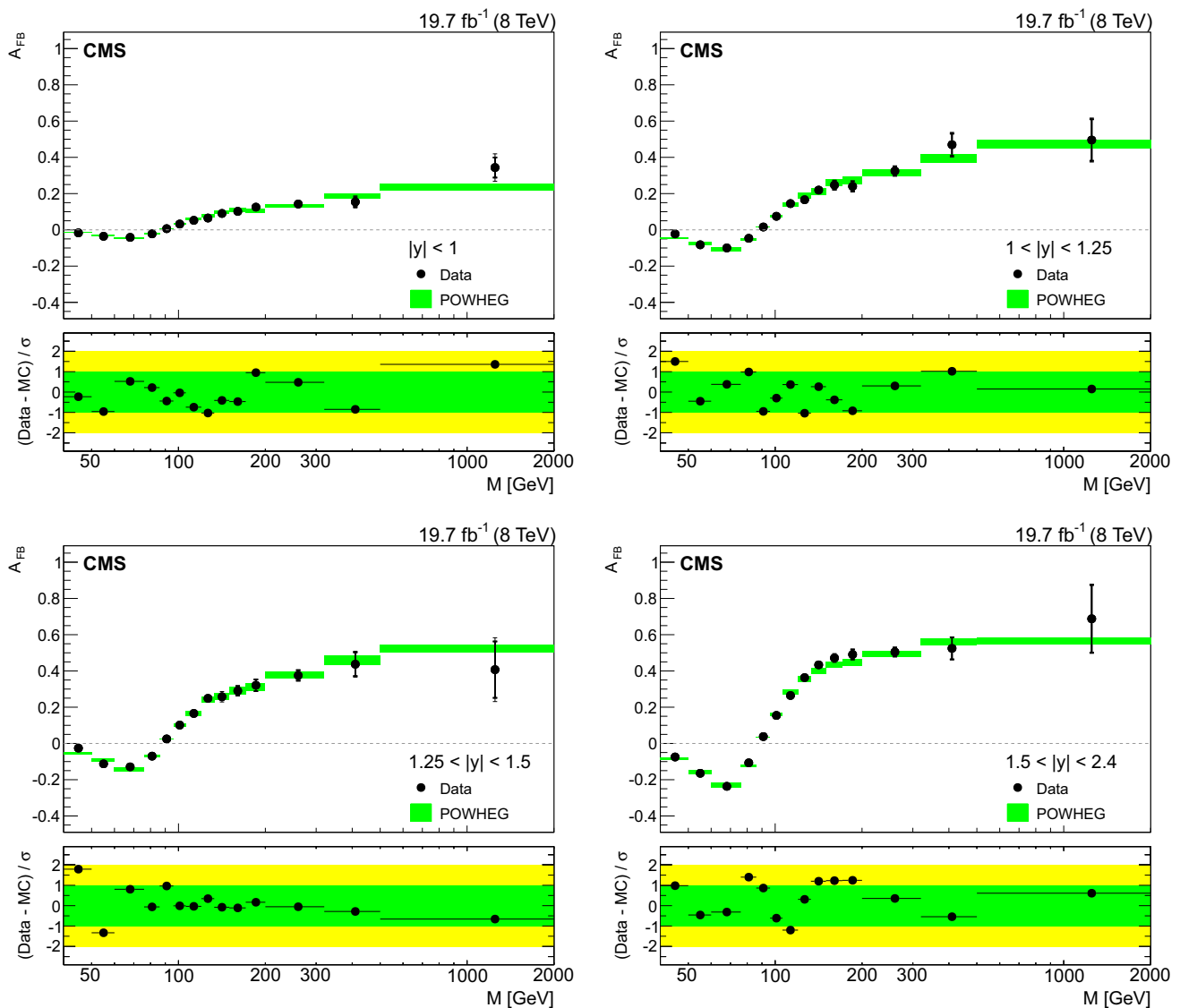
Fig. 4 The combined ( \mu^+\mu^- and e^+e^- ) unfolded A_{FB} distributions in the four central rapidity regions. The statistical (thick vertical bar) and statistical plus systematics (thin vertical bar) uncertainties are presented. The measurements are compared with the prediction
