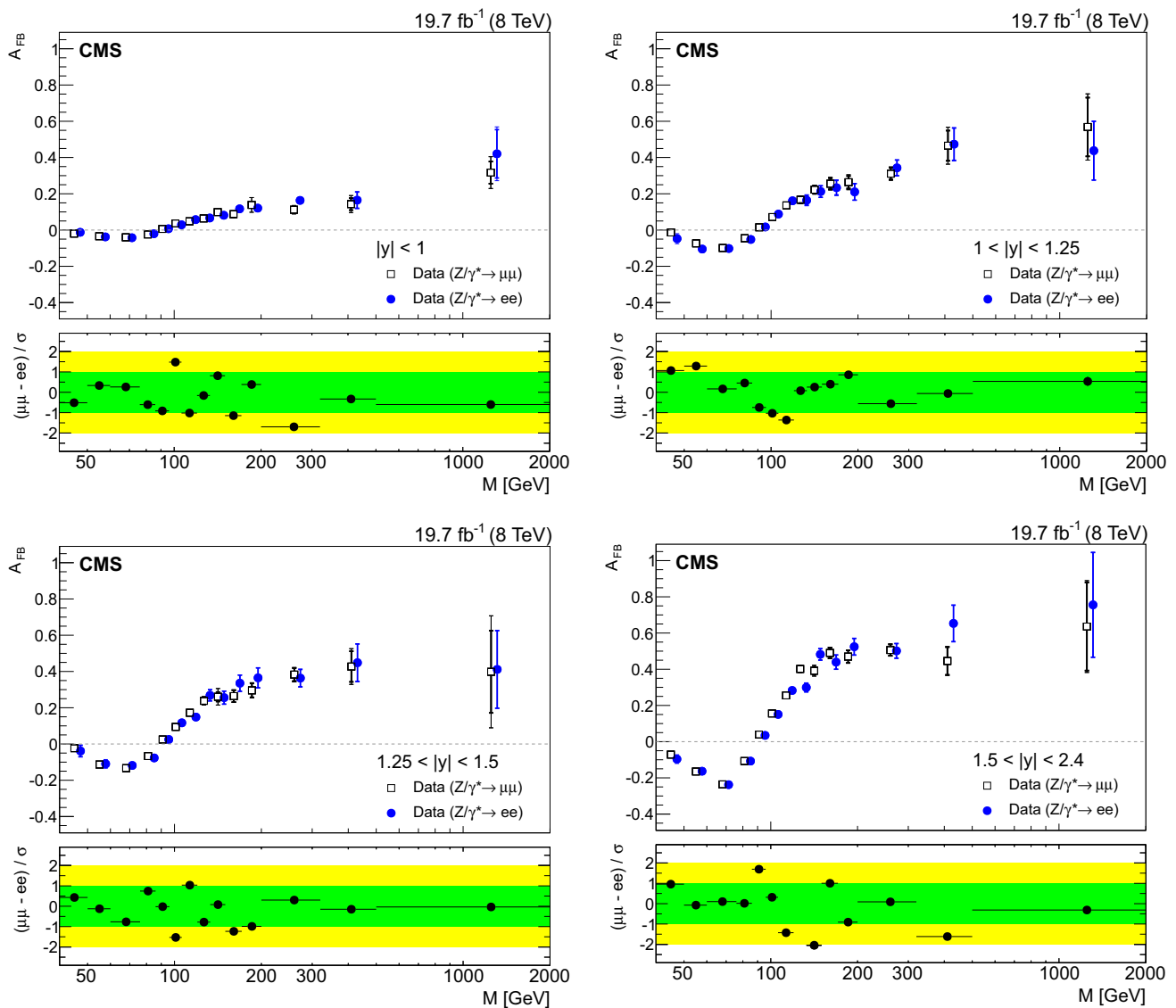
Fig. 3 The unfolded A_{FB} distributions for muons (open squares) and electrons (solid circles) for the four central rapidity regions. The statistical (thick vertical bar) and statistical plus systematic (thin vertical bar) uncertainties are presented. The solid circles are shifted slightly
