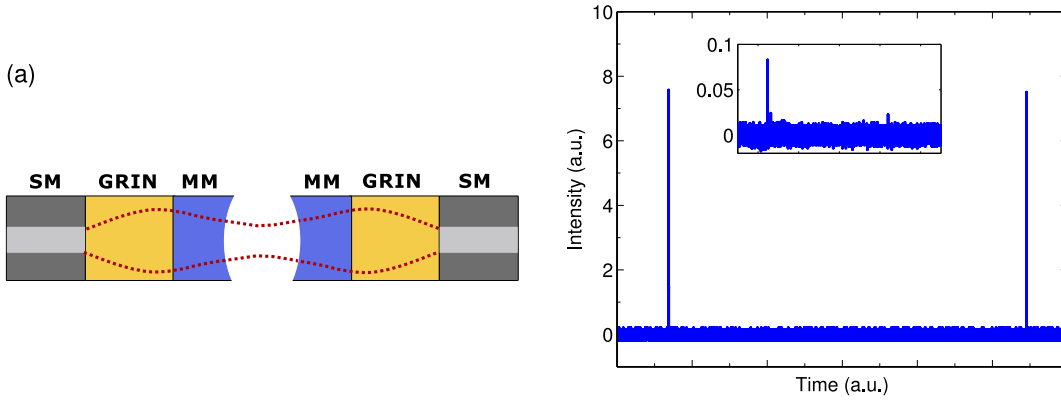
Figure 5. (a) Schematic of a FA-FA system where mode matching fiber assemblies are used as the input as well as the output of the FFPC. (b) Transmission spectrum of the FA-FA system as the cavity is scanned by a piezo actuator over approximately one FSR. The inset shows details of the higher order mode transmission.
