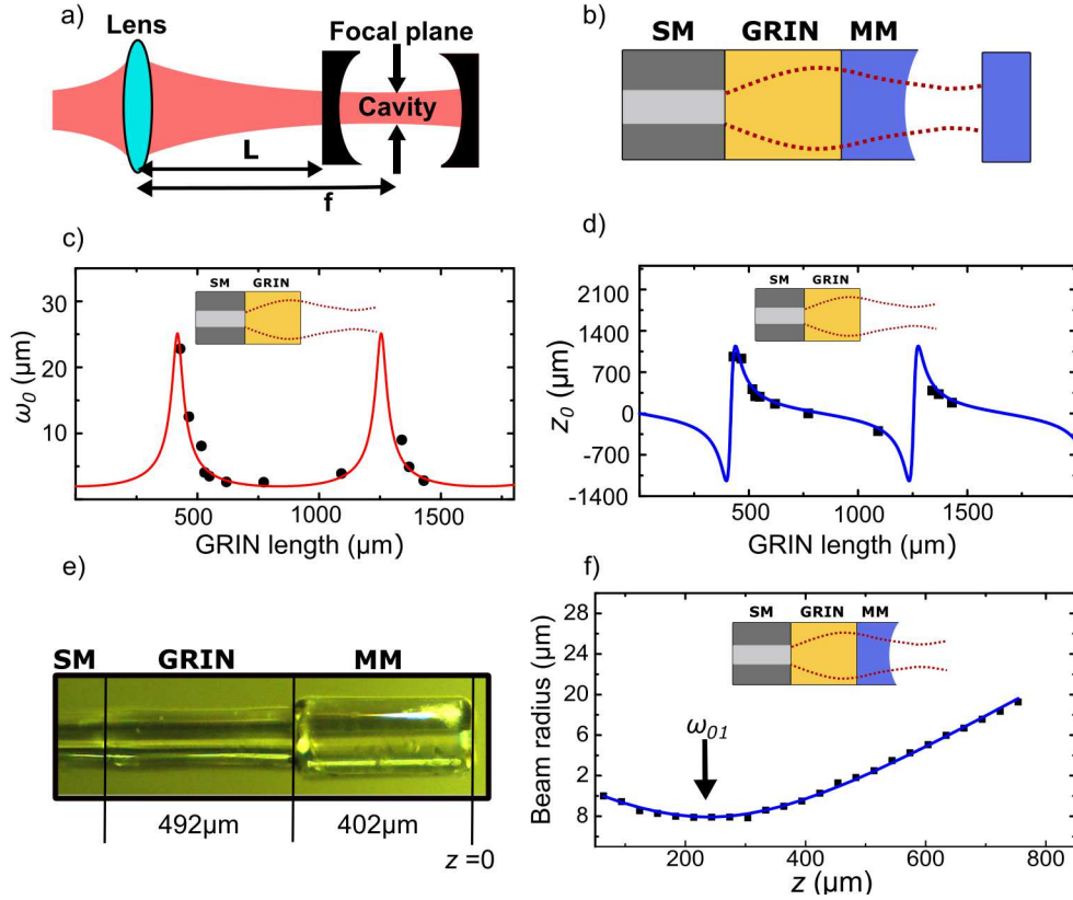
Figure 1. a) Mode matching between an optical cavity and a laser beam in free space. b) Design of the mode matching fiber assembly. c) and d) Waist size ( \omega_0 ) and waist position ( z_0 ) with respect to end facet of GRIN fiber as a function of GRIN fiber length for a simple SM-GRIN unit. Solid lines are calculated results using the ray matrix transformation method with a fitted value of gradient constant ( g ) of 3.77 \text{ mm}^{-1} . e) Actual mode matching fiber assembly (FA) with the GRIN and MM fibers of length 492 \mu\text{m} and 402 \mu\text{m} respectively. The lengths of the respective fibers determine the mode waist ( \omega_{01} ) and waist position ( z_{01} ) of mode at the output of the FA (SM-GRIN-MM). f) Mode radius of the output from the FA, where z=0 is the laser ablated end facet of the MM fiber. Waist size ( \omega_{01} ) of 8.1 \mu\text{m} at z_{01} = 230 \mu\text{m} is obtained by fitting the data with the propagation of a Gaussian beam.
