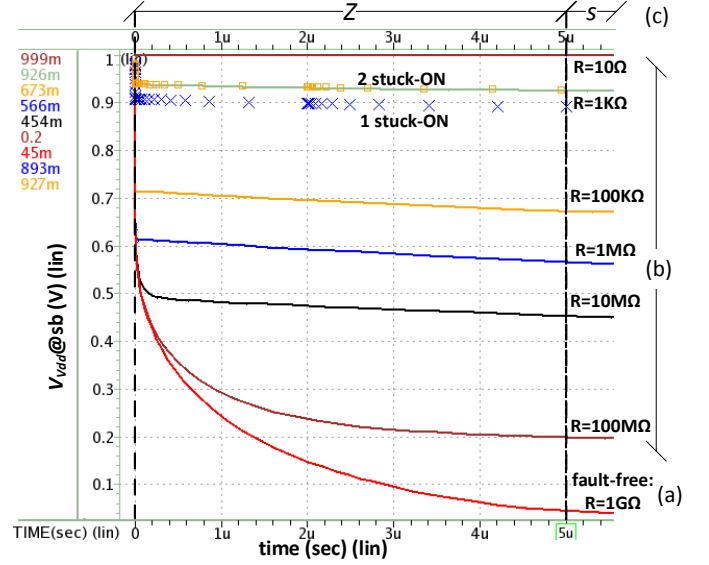
Fig. 9. AC analysis of bridges at power rails and stuck-on power switches
