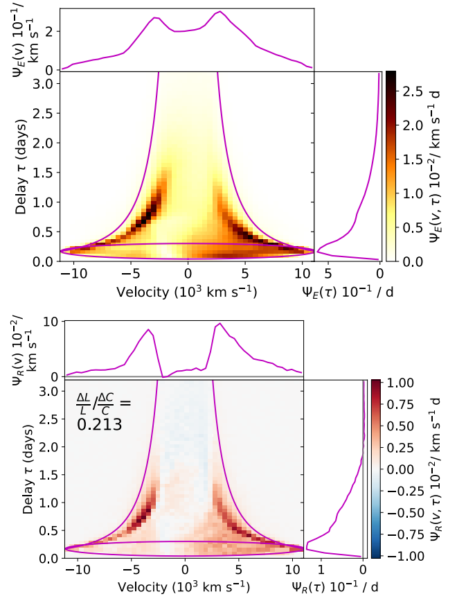
Figure 12. The velocity-resolved EWRf (upper) and response function (lower) for C IV in the Seyfert model, shown for time delays up to 3.2 days. The violet lines illustrate the function edges for a Keplerian disc at the wind launching radius, and the v \propto \tau^{-1/2} "virial flow" envelope.
