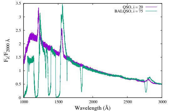
Figure 4. Spectra produced for the disc wind model of Matthews et al. (2016) , viewed along QSO ( i = 20^\circ ) and BALQSO ( i = 75^\circ ) sightlines. Both spectra have been normalised to unity at 2000 Å.
