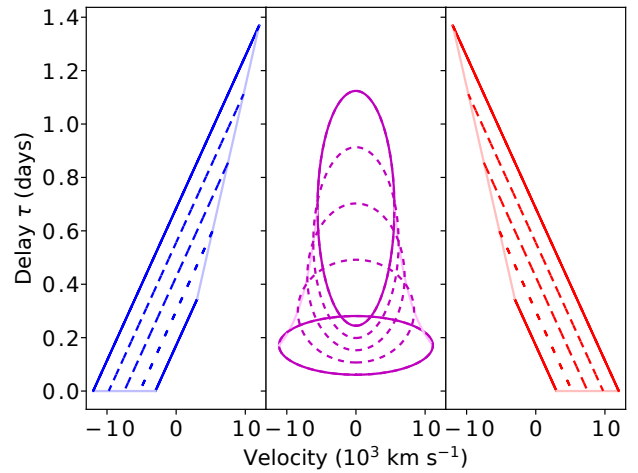
Figure 3. Outline response functions for Hubble-type spherical outflow (left), a rotating Keplerian disc viewed at a 20^\circ angle (centre), and Hubble-type spherical inflow (right). Winds extend from r_{min} = 20r_g to r_{max} = 200r_g for an AGN of mass 10^7 M_\odot . Hubble out/inflows have V(r_{min}) = \pm 3 \times 10^3 \text{ km s}^{-1} . Solid lines denote the response from the inner and outer edges of the winds, dotted lines from evenly-spaced shells within the wind. Pale lines describe the edge of the velocity-delay shape of the response function.
