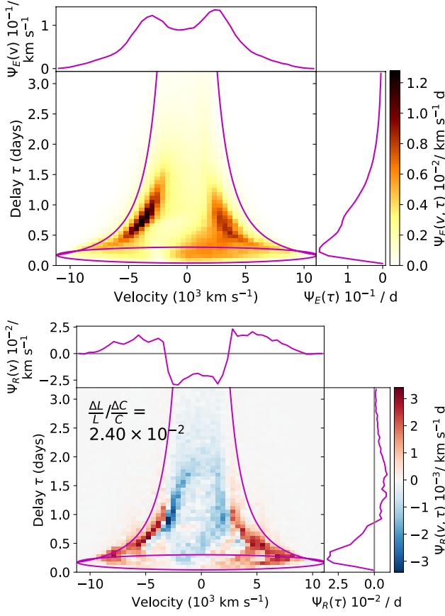
Figure 11. The velocity-resolved EWRf (upper) and response function (lower) for H \alpha in the Seyfert model, shown for time delays up to 3.2 days. The violet lines illustrate the function edges for a Keplerian disc at the wind launching radius, and the v \propto \tau^{-1/2} "virial flow" envelope.
