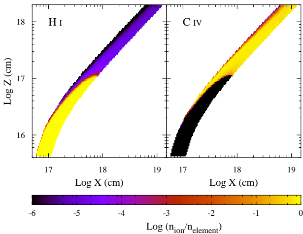
Figure 7. The H I and C IV ionization fractions within the wind in the QSO model.
