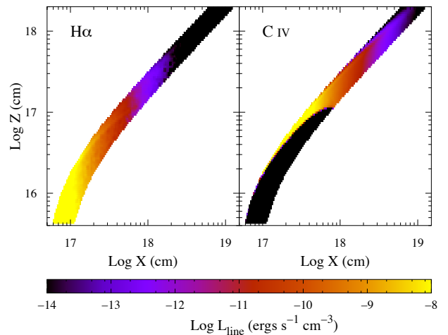
Figure 8. The line emissivity distribution for the H \alpha and C IV lines in the QSO model.
