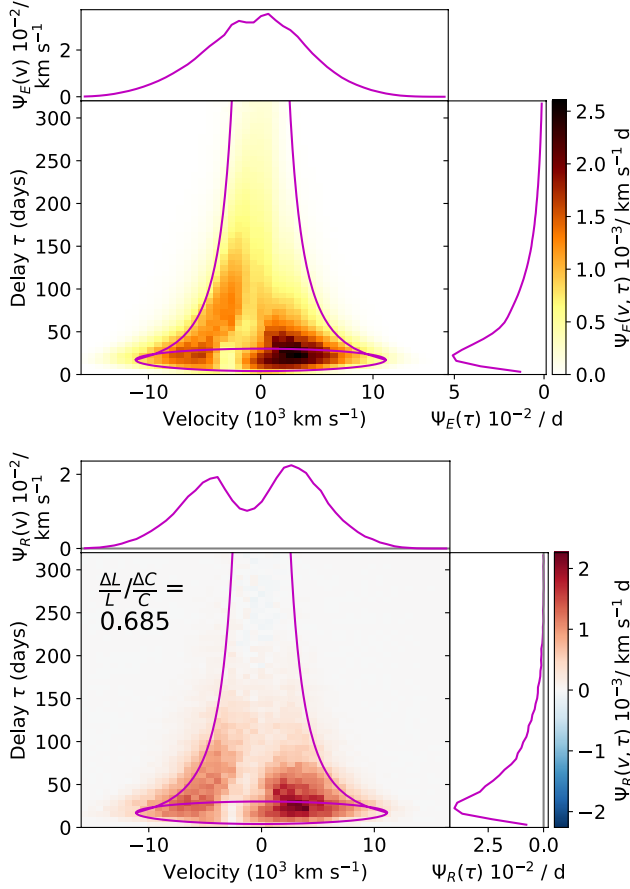
Figure 5. The velocity-resolved EWRf (upper) and response function (lower) for H \alpha in the QSO model, shown for time delays up to 320 days. The violet lines illustrate the function edges for a Keplerian disc at the wind launching radius, and the v \propto \tau^{-1/2} "virial flow" envelope. Note that the velocity-integrated line response is weakly negative at low velocities beyond \tau \gtrsim 220 days.
