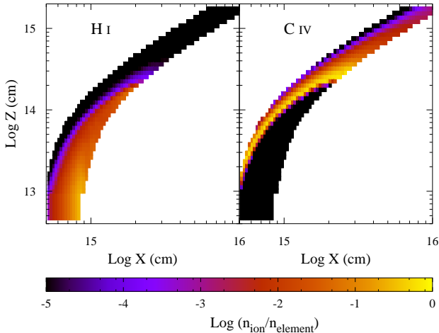
Figure 13. The H I and C IV ionization fractions within the wind in the Seyfert model. This graph shows a smaller region of the wind than figure 7 as the outflow is overionized in the Seyfert model and does not show emission in common RM lines.
