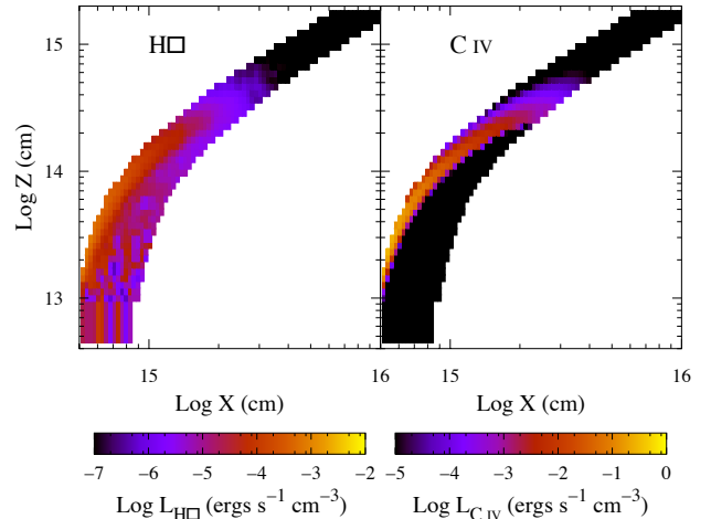
Figure 14. The line emissivity distribution for the H \alpha and C IV lines in the Seyfert model. This graph shows a smaller region of the wind than figure 8 as the outflow is overionized in the Seyfert model and does not show emission in common RM lines.
