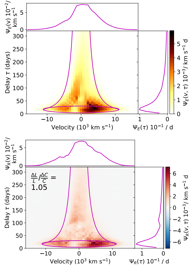
Figure 6. The velocity-resolved EWRf (upper) and response function (lower) for C IV in the QSO model, shown for time delays up to 320 days. The violet lines illustrate the function edges for a Keplerian disc at the wind launching radius, and the v \propto \tau^{-1/2} "virial flow" envelope.
