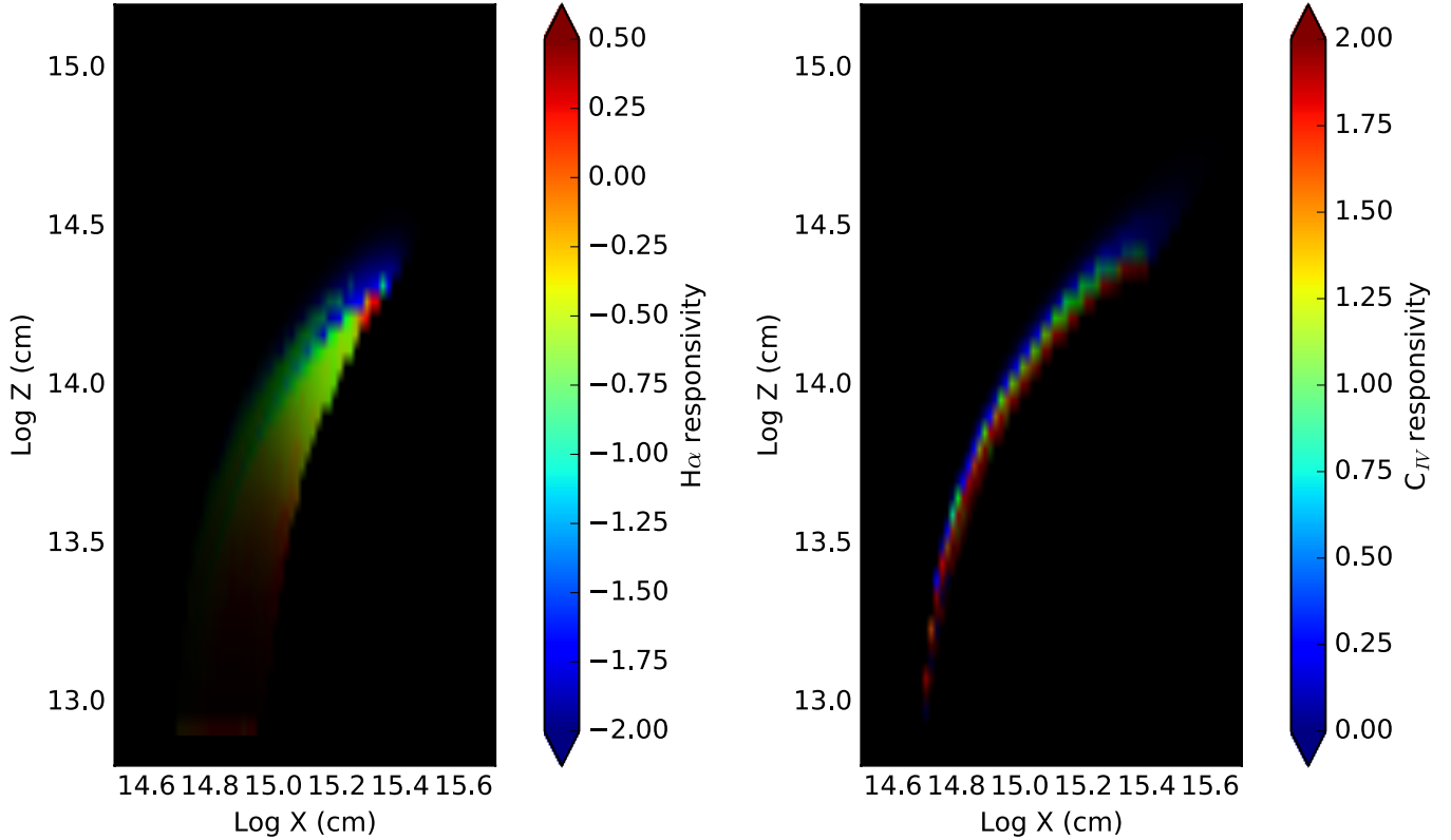
Figure 15. The local responsivity \eta for H \alpha (left) and C IV (right). Colour indicates responsivity, brightness indicates local emissivity. The brightest cells on the figure are in the upper 99.9% of cells for line emission; other cell brightnesses are scaled linearly to this value.
