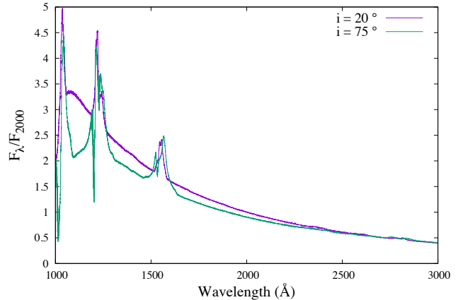
Figure 9. Spectra for Seyfert model along above wind i = 20^\circ and through-wind (BAL-equivalent in QSO model) i = 75^\circ sightlines, for comparison to Figure 4, normalised to flux at 2000 Å. Only very faint BAL features are apparent for BALQSO-like sightlines.
