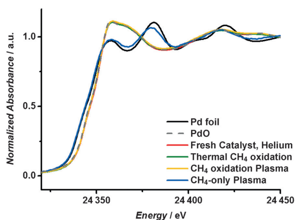
Figure 2. Normalized XANES spectra of the Pd foil reference, the PdO reference, the fresh catalyst (sample 1) under helium gas, the catalyst during the thermal \text{CH}_4 oxidation reaction, the catalyst during plasma-activated \text{CH}_4 oxidation, and during \text{CH}_4 -only reaction under plasma conditions.
