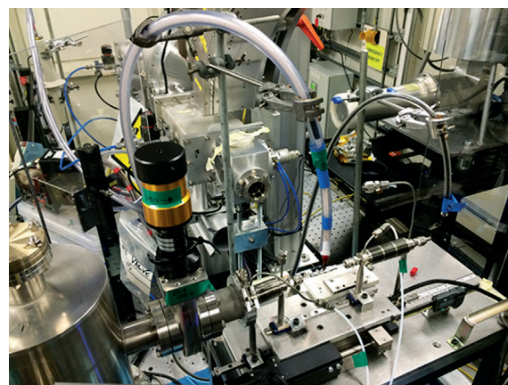
Figure 1. Setup for in situ measurements using XAFS spectroscopy coupled with MS for \text{CH}_4 oxidation using plasma.
