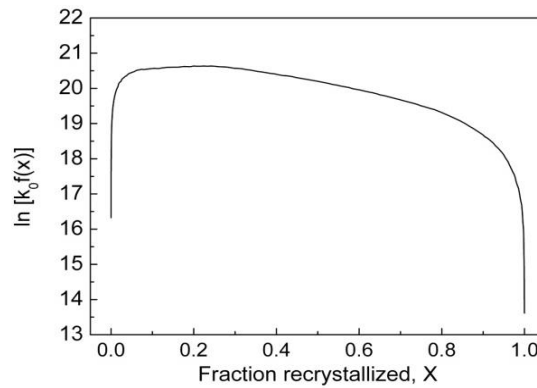
Figure 3 Plot of \ln [k_0 f(x)] versus recrystallized fraction X .
