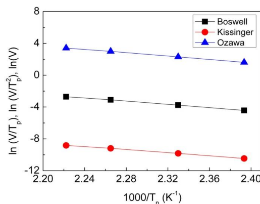
Figure 4 Plots of \ln (V/T_p) , \ln (V/T_p^2) and \ln (V) against 1000/T_p of Mg-1.44 wt.% Ce alloy processed by HPT to 1/2 turn
