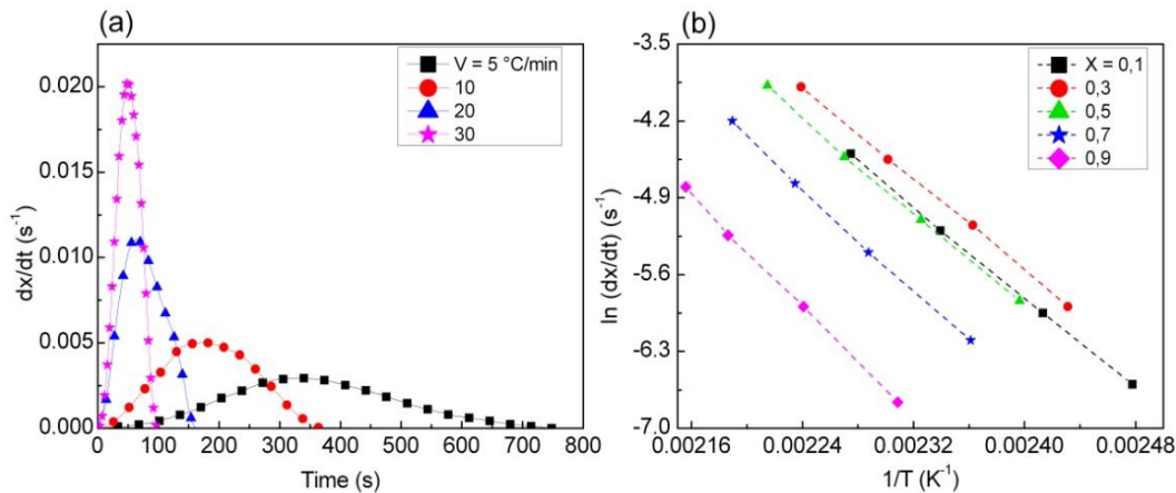
Figure 2 a) Rate of recrystallization process versus time, b) Plot of \ln (dX/dt) versus 1/T of Mg-1.44 wt.% Ce alloy processed by HPT to 1/2 turn
