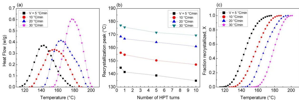
Figure 1 a) DSC curves of an exothermic peak records to the recrystallization process of Mg-1.44 wt.% Ce alloy processed by HPT to 1/2 turn, b) Evolution of recrystallization temperature peak of Mg-1.44 wt.% Ce as function of number of HPT turns and c) Fraction recrystallized, X versus temperature of Mg-1.44 wt.% Ce alloy processed by HPT to 1/2 turn.
