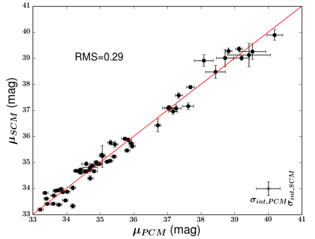
FIG. 7.— Comparison distance modulus obtained using the PCM (x-axis) and the SCM (y-axis). The red line shows x = y . Note that the error bars do not include the intrinsic scatter ( \sigma_{int} ) of each method which are represented by the cross on the bottom right of the figure.
