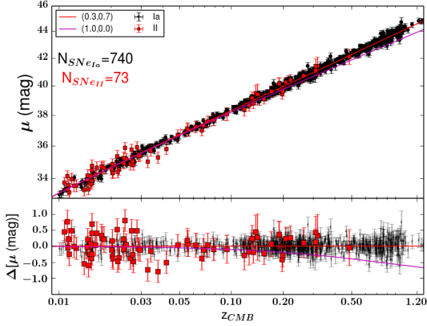
FIG. 10.— Combined Hubble diagram using SNe Ia from Betoule et al. (2014) and SNe II. The red squares are for the SNe II (using the PCM) and the black dots for the SNe Ia. Note that distance modulus errors for both methods include the intrinsic dispersion. The red line the Hubble diagram for the \Lambda CMB ( \Omega_m=0.3 and \Omega_\Lambda=0.7 ) and in magenta line an Einstein-de Sitter cosmological model ( \Omega_m=1.0 and \Omega_\Lambda=0.0 )
