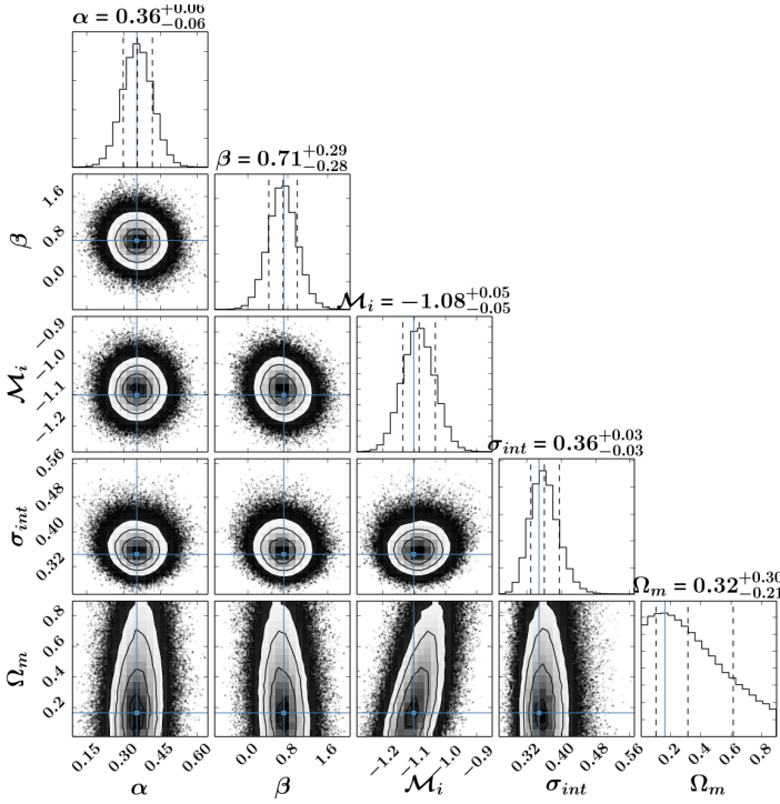
FIG. 2.— PCM: Corner plot showing all the one and two dimensional projections. The blue lines are the values obtained using only one likelihood minimisation. Contours are shown at 1, 2, and 3 sigmas. The five free parameters are plotted: \alpha , \beta , M_i , \sigma_{int} , and \Omega_m . To make this figure we use the corner plot package (triangle.py v0.1.1. Zenodo. 10.5281/zenodo.11020)
