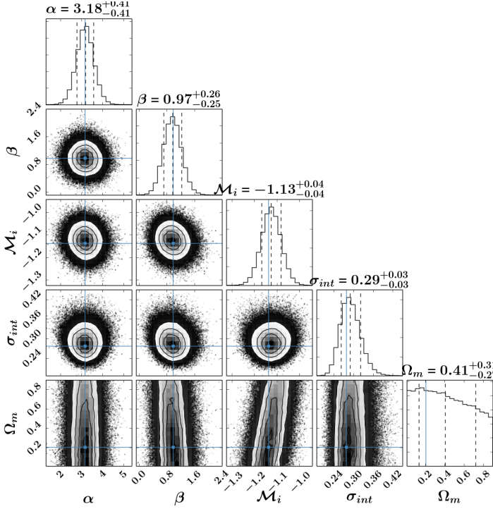
FIG. 5.— SCM: Corner plot showing all the one and two dimensional projections. The blue lines are the values obtained using only one likelihood minimisation. Contours are shown at 1, 2, and 3 sigmas. The five free parameters are plotted: \alpha , \beta , \mathcal{M}_i , \sigma_{int} , and \Omega_m .
