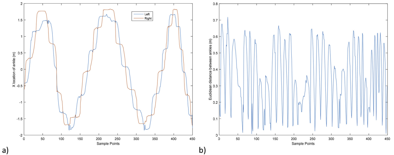
Fig. 2. a) Illustrative left and right ankle x coordinates extracted from walking sequence, b) Euclidean distance between ankle x coordinates.
