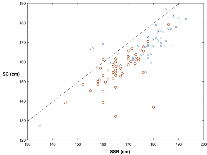
Fig. 4. Self-reported stature vs calculated stature. The dashed line shows the ideal correlation between the two variables. (blue crosses = male subjects, red circles = female subjects). (For interpretation of the references to colour in this figure legend, the reader is referred to the web version of this article.)
