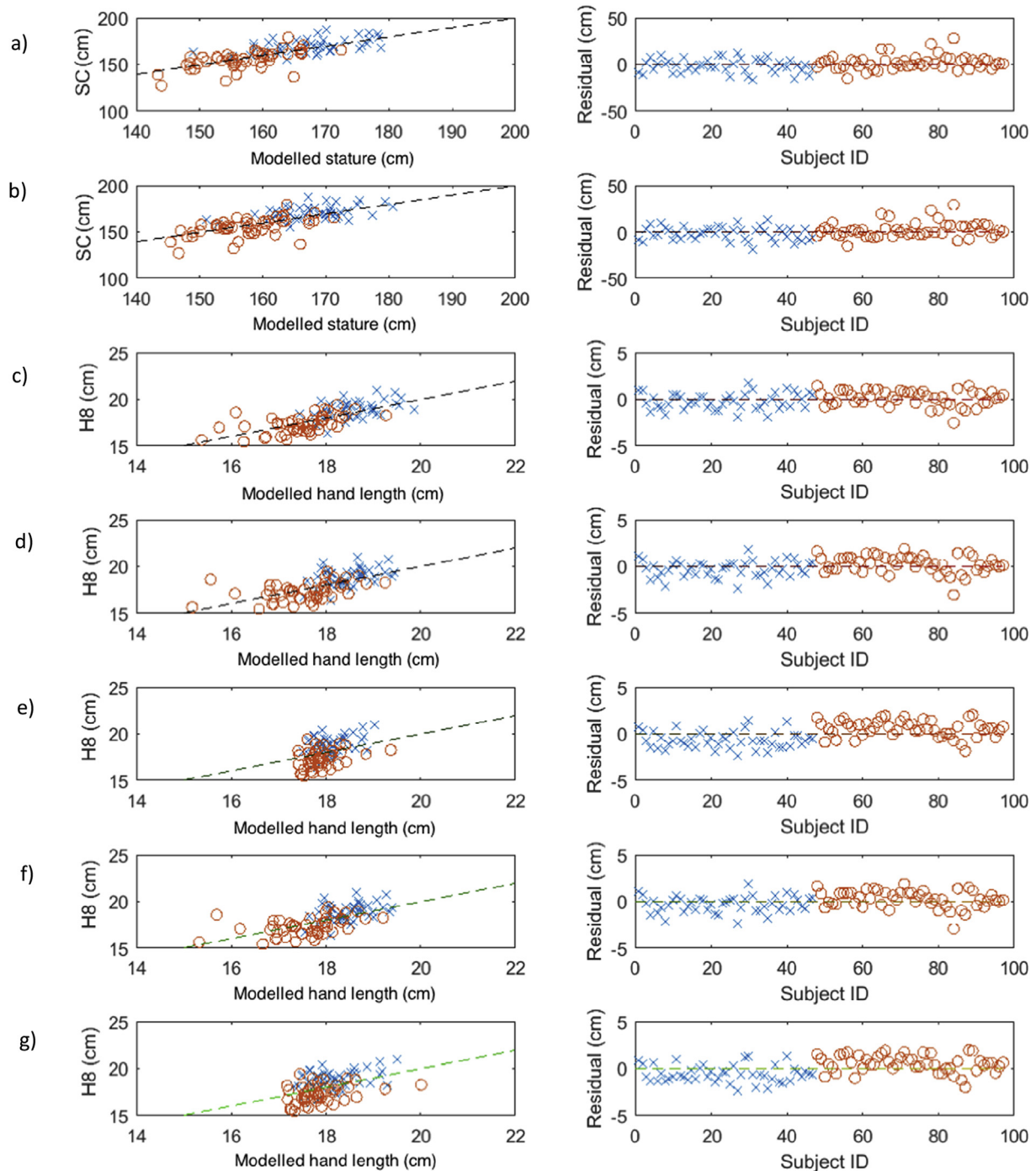
Fig. 5. Modelled relationships and individual subject residuals for each of the seven scenarios in Table 7 (blue crosses = male subjects, red circles = female subjects). (For interpretation of the references to colour in this figure legend, the reader is referred to the web version of this article.)
