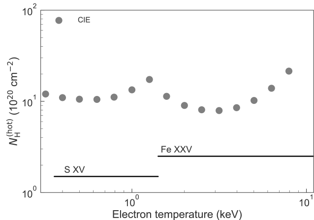
Fig. 4. 3\sigma statistical upper limits of the hydrogen-equivalent extinction column ( N_{\text{H}}^{\text{(not)}} ) by the CIE plasma for the assumed electron temperature. The name of ions giving the strongest absorption line at each temperature is shown at the bottom
