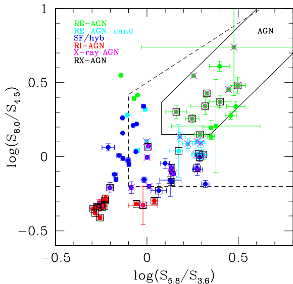
Figure 9. The IRAC colour-colour diagram for the 77 5.5 GHz selected radio sources detected at all IRAC bands, highlighting X-ray AGN (magenta crosses) and radio-excess sources (black squares).
