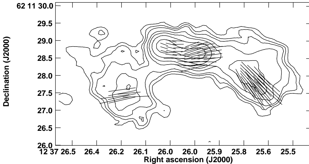
Figure 4. Polarisation vectors with directions along the apparent electric field and lengths proportional to the degree of polarisation at 5.5 GHz, superimposed on the radio contours of total intensity across J123726+621128 at the same frequency. The angular resolution is \simeq 0.5 arcsec FWHM.
