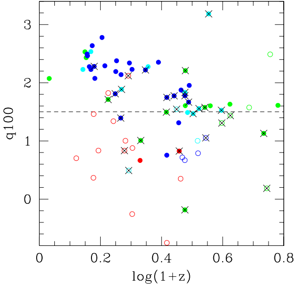
Figure 10. The q_{100} = \log(S_{100\mu\text{m}}/S_{1.4\text{GHz}}) as a function of redshift for the 5.5 GHz radio-selected sample with full IRAC detection. Symbols are the same as in Fig.8, except that open symbols are used for sources that have only an upper limit at 100\mu\text{m} .
