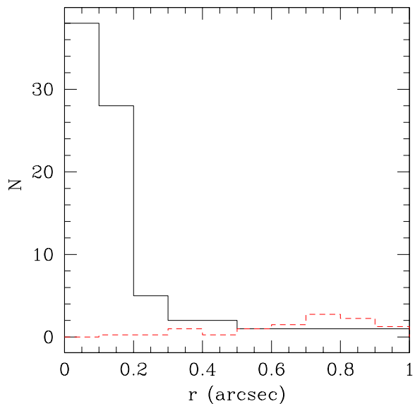
Figure 5. Separation of the nearest K_s -band counterparts from the radio sources (solid black line), and by shifting the radio sources by 1 arcmin in four directions and repeating the matching (dashed red line).
