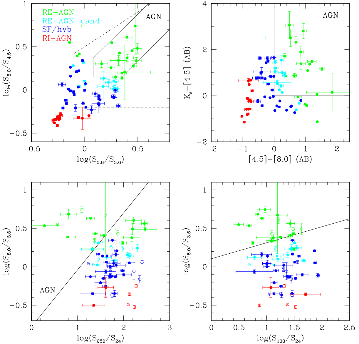
Figure 8. The four IR colour-colour plots used to classify the 5.5 GHz radio sources in the GOODS-N field. In each panel different colours are used to identify different classes of sources based on the classification obtained by combining all the four IR plots: RE-AGN are shown in green, RE-AGN-candidates in cyan, RI-AGN in red, and the remaining sources (SF/hyb galaxies) in blue. Top-Left: IRAC colour-colour plot, the dashed-line wedge shows the AGN selection region from Lacy et al. (2007) , while the smaller area enclosed by a solid-line is the revised wedge from Donley et al. (2012) , used in this paper. Top-Right: KI colour-colour plot ( Messias et al. 2012 ). The region populated by AGN is delimited by the solid line defined as K_s - [4.5] > 0 and [4.5] - [8.0] > 0 . Magnitudes are in the AB photometric system. Bottom-Left: IR colour-colour plot showing \log(S_{8.0}/S_{3.6}) versus \log(S_{250}/S_{24}) . The line separate RE-AGN (above the line) from star-forming or passive galaxies (below the line), according to Kirkpatrick et al. (2012, 2013) Bottom-Right: IR colour-colour plot showing \log(S_{8.0}/S_{3.6}) versus \log(S_{100}/S_{24}) . The line separates RE-AGN (above the line) from star-forming or passive galaxies (below the line), according to Kirkpatrick et al. (2012, 2013) . In the two lower plots, empty symbols refer to 100 \mu\text{m} and 250 \mu\text{m} upper limits.
