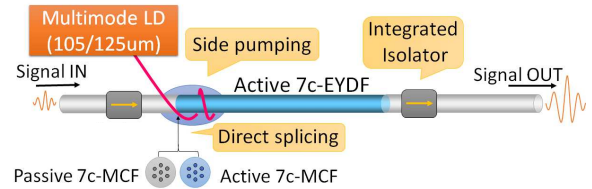
Fig. 2. Schematic diagram of the internal structure of a MC-EYDFA. The position of the integrated isolator in the MC-EYDFA depends on the role of the amplifier in the system. A pre-amplifier has the isolator at the input of the MC-EYDFA, whereas a post-amplifier has it placed at the output.
