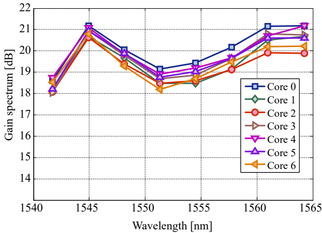
Fig. 5. Gain spectrum of the 7-core MC-EYDFA for an MMPD current of 2 A. The gain spectrum takes into account the insertion loss of one integrated multicore isolator.
