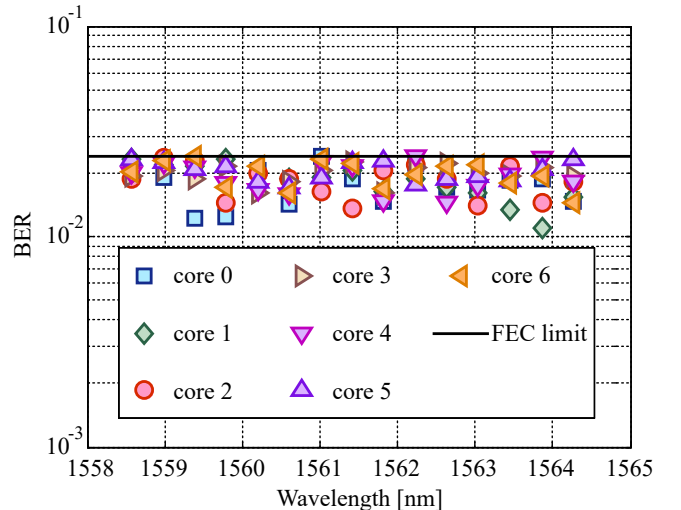
Fig. 9. BER of the 200 Gbit/s 16-QAM test channel over all 15 channels per core after a transmission distance of 720 km.
