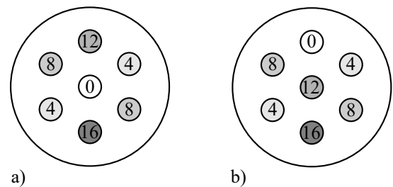
Fig. 6. Relative delay lines in meters with respect to a given core to de-correlate signals between optical waveguides: a) with respect to the middle core, and b) with respect to one of the outer cores.
