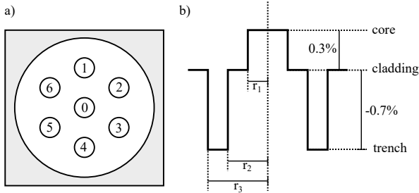
Fig. 1. a) Hexagonal waveguide layout and core identifiers of the 7-core MCF used in the experiments. b) Refractive index profile of the 7-core MCF.
