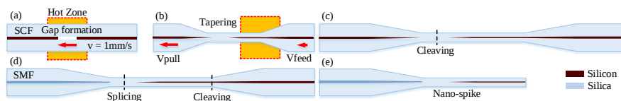
Fig. 1. Steps of fabrication. (a) Void gap formation in the core of an as-drawn SCF after heat-polishing process. (b) Tapering of the void gap in the core results in a silicon-free region with a CaO/ \text{SiO}_2 core, and a nano-spike. (c) Cleaving of the tapered SCF. (d) Splicing the SCF with a tapered SMF and final cleaving at the other end. (e) An SMF-SCF device with a nano-spike.
