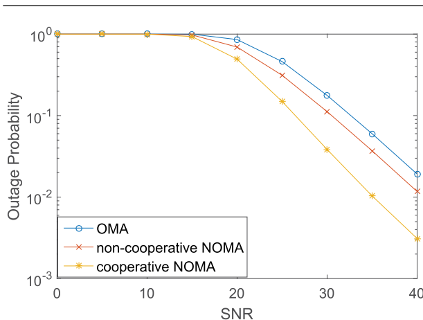
Fig. 9. Performance comparison between cooperative NOMA and noncooperative NOMA. The BS is located at (0, 0), user m is located at (4, 0), user n is located at (1, 0), the path loss exponent is 3, and the power allocation coefficient for user m and user n is (0.8, 0.2). The targeted data rate is 1 bits per channel use (BPCU).
