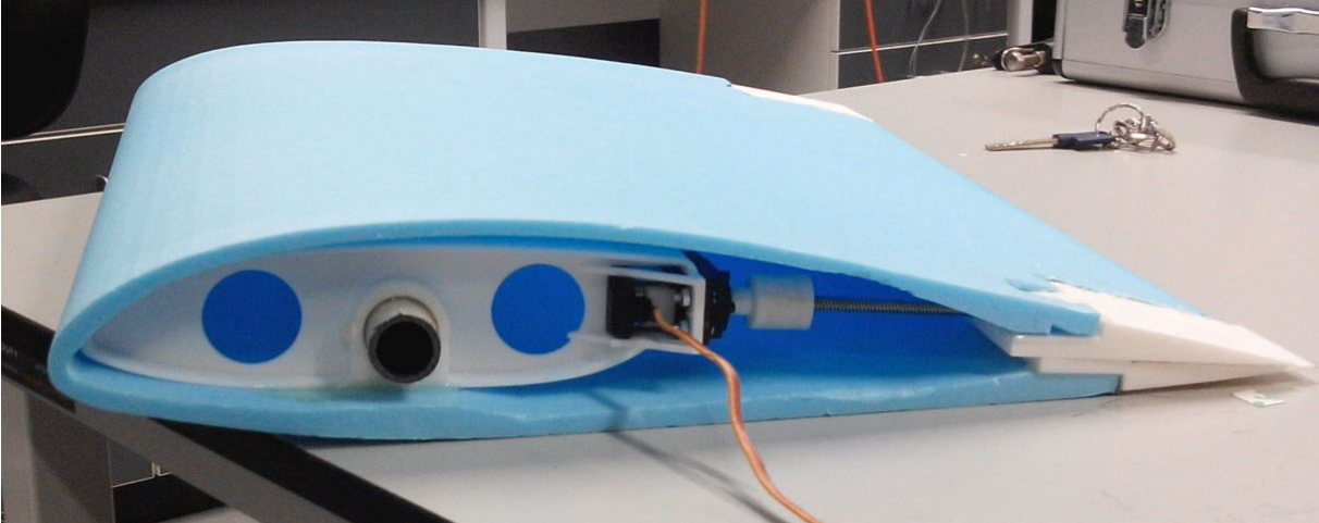
Figure 3 – morphing mechanism in situ in test section.
