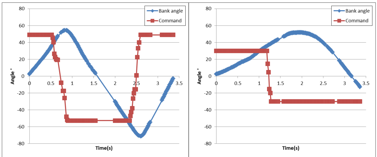
Figure 22 – typical bank and command angle for conventional (a) and morphing wings (b).
