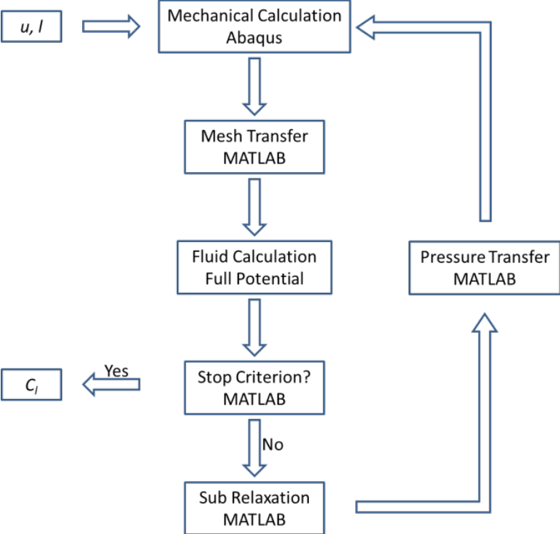
Figure 13 – Aeroelastic analysis algorithm
