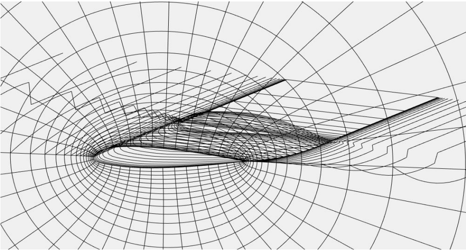
Figure 11 – 3D mesh of the deformed wing in FP.
