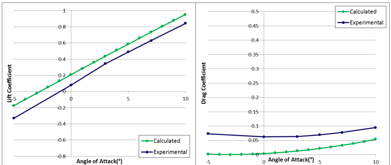
Figure 19 – lift (a) and drag (b) coefficient at 24m/s; morphing activated.
