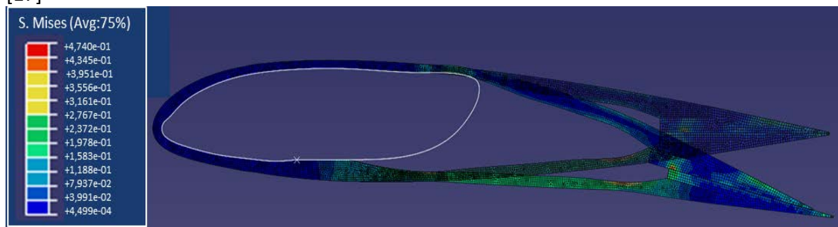
Figure 10 – deformed and un-deformed mesh of the Abaqus finite element analysis model.
