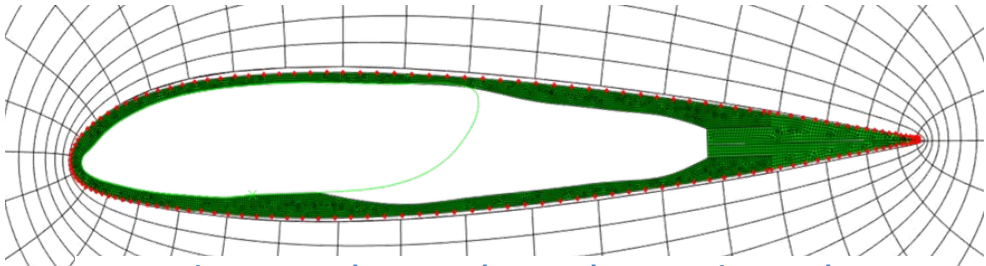
Figure 14 – Abaqus and FP meshes superimposed
