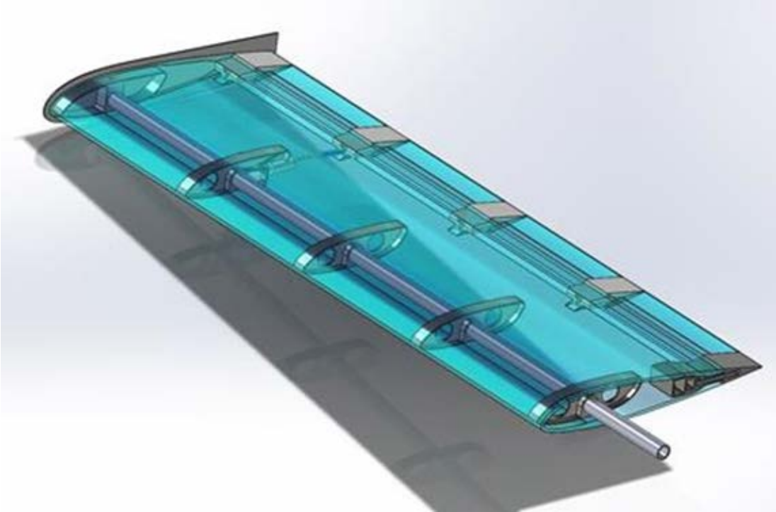
Figure 2 – CAD model of the morphing wing – note actuator on fourth rib.
