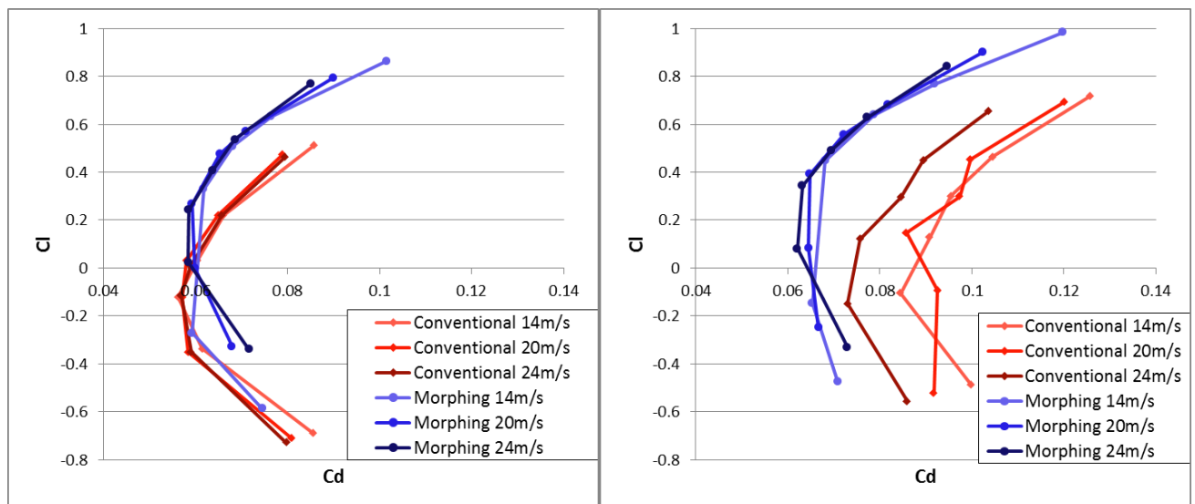
Figure 20 – experimental Lift Drag coefficient Comparison, un-activated (a), activated (b).
