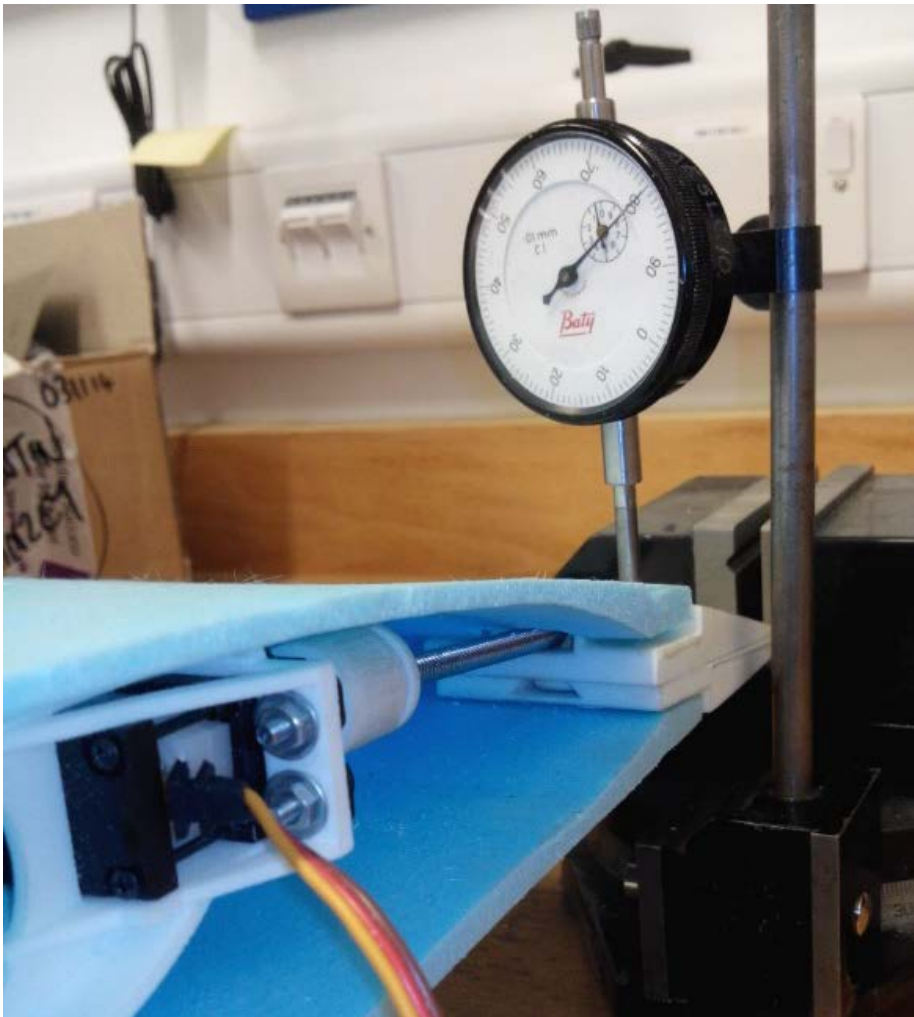
Figure 8 – experimental measurement of part deflection on short test section.
