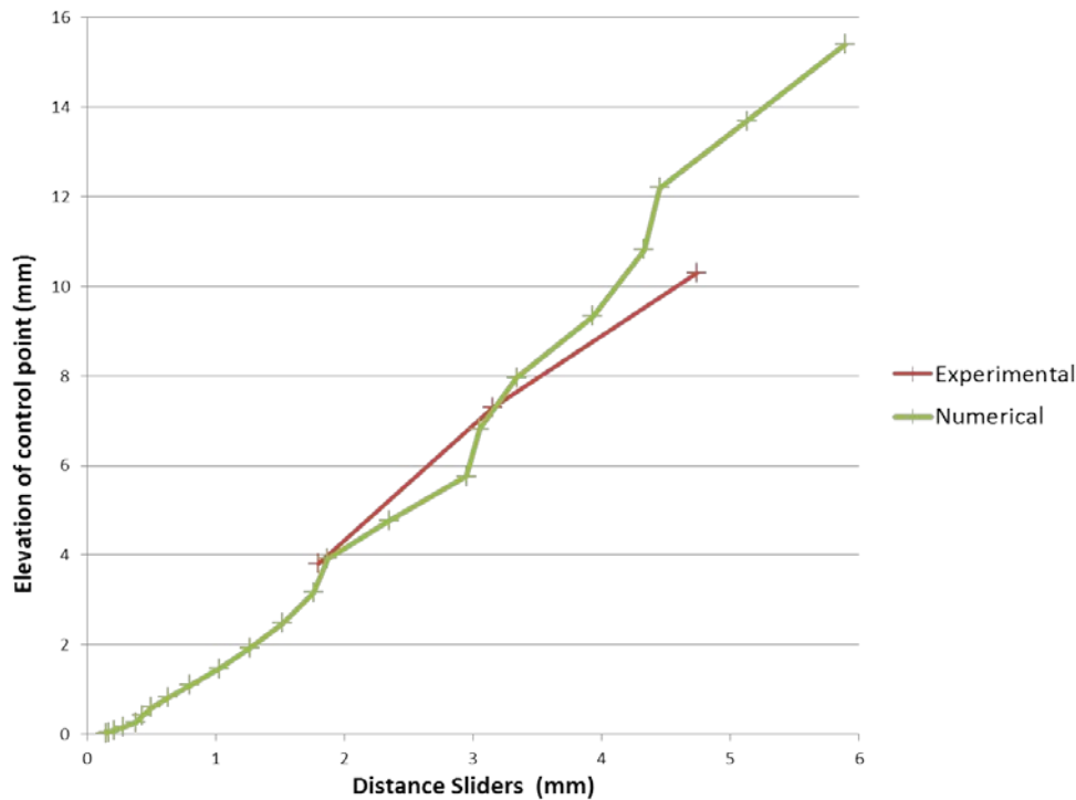
Figure 9 – comparison of computational and experimental deflections.
