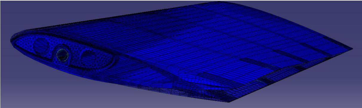
Figure 7 – 3D deformed and un-deformed wing superimposed.
