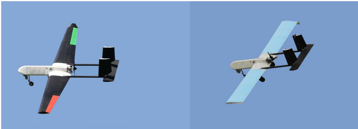
Figure 21 – UAV Mark IV flying with conventional wings (a) and morphing wings (b).
