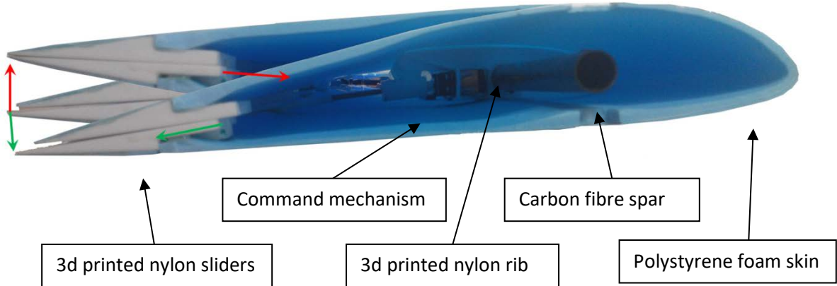
Figure 1 – superimposed profiles of the morphing wing during movement.
