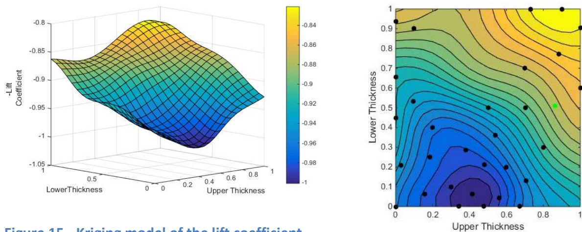
Figure 15 - Kriging model of the lift coefficient
