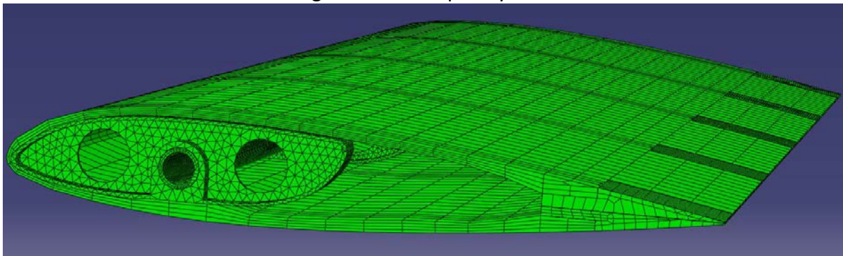
Figure 5 – 3D Abaqus mesh
