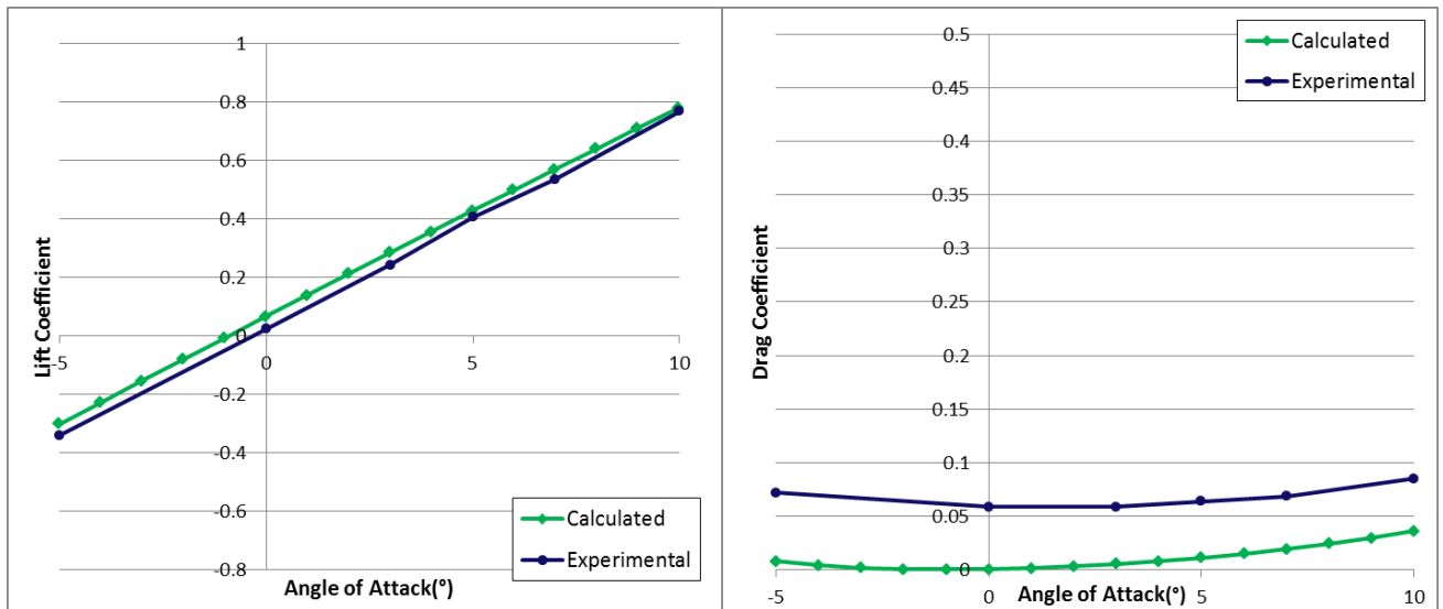
Figure 18 – lift (a) and drag (b) coefficient at 24m/s; no morphing.
