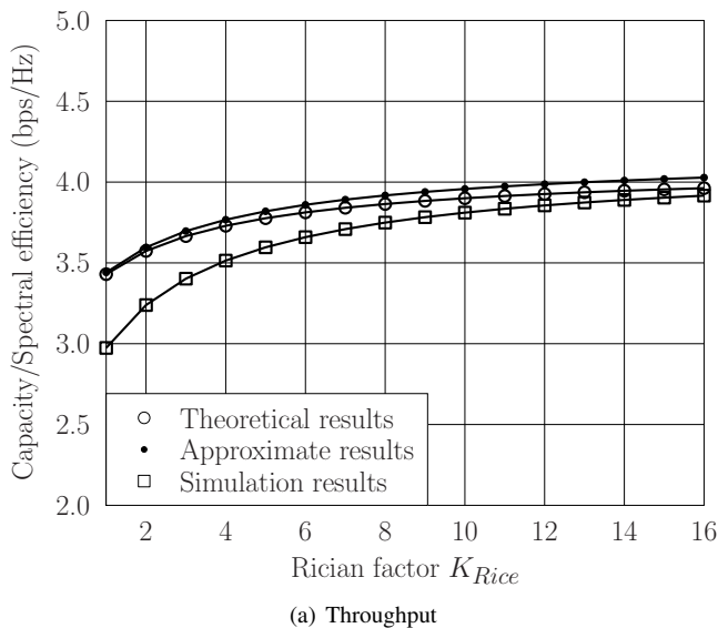
Fig. 9. (a) The achievable throughput per DRA as a function of the Rician factor K_{Rice} , and (b) The CCDFs of the simulated throughputs per DRA for different values of K_{Rice} . The distances between the interfering aircraft and the desired receiving aircraft are uniformly distributed within the range of [d_{b^*}^a, D_{max}] . The rest of the parameters are specified in Table III.
