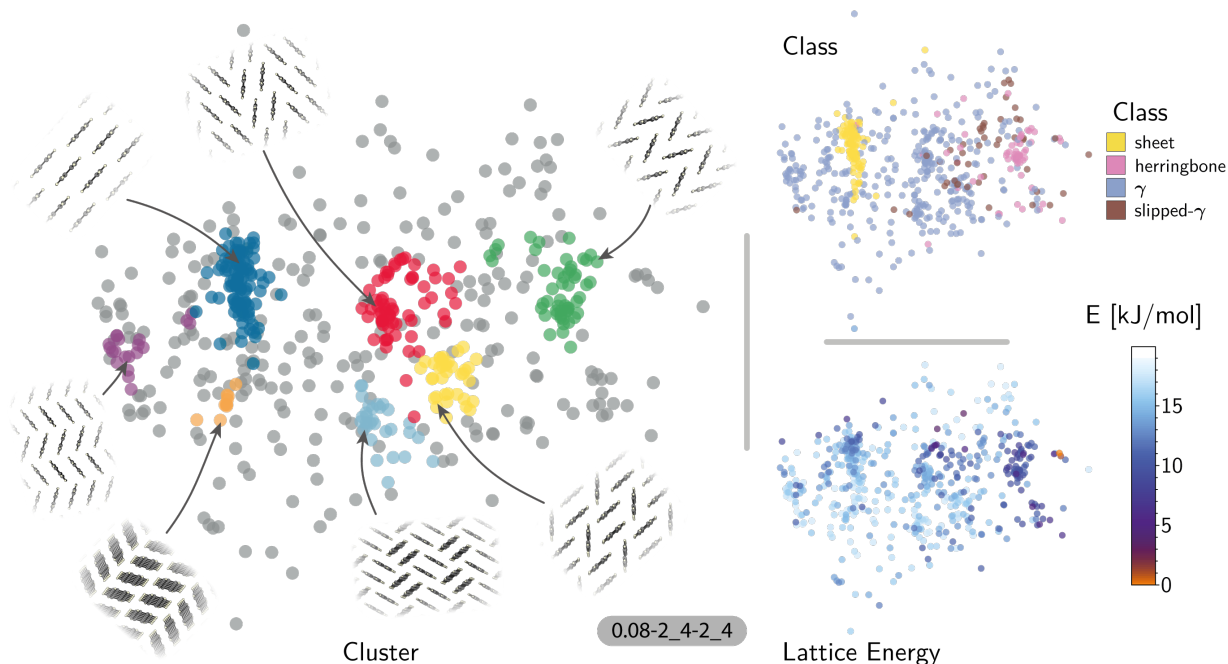
Fig. 3 Sketch-map representations of the pentacene crystal structure landscape's similarity matrix (projection parameters shown follow the scheme \sigma_{map-A\_B-a\_b} ). The atomic configurations are color-coded according to their relative lattice energy (bottom right), class following the heuristic classification (top right) and cluster index (gray structures do not belong to a cluster) found using HDBSCAN* on the similarity matrix (left). The structural pattern of each cluster is illustrated from a view down the short edge of pentacene.
