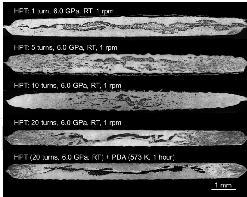
Fig. 1 The vertical cross-sections of the Al-Mg system after HPT under a pressure of 6.0 GPa at room temperature for, from the top, 1, 5 and 10 turns [13-15] and 20 turns plus 20 turns followed by PDA [16].
