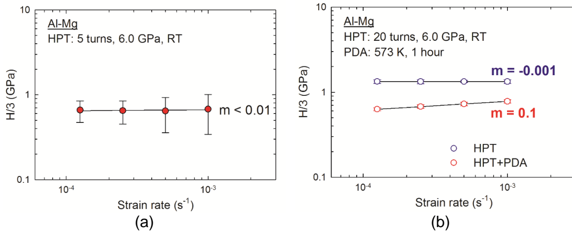
Fig. 7 Variations of the strain rate sensitivity with increasing strain rate for the disk edges of the Al-Mg system after HPT for (a) 5 turns [14,22] and (b) 20 turns and after HPT and PDA [16].
