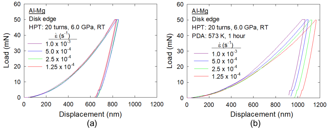
Fig. 6 Representative load-displacement curves for the Al-Mg disk edges after (a) HPT for 20 turns and (b) HPT and PDA when measuring at four strain rates from 1.0 \times 10^{-3} to 1.25 \times 10^{-4} s -1 under a predetermined maximum peak load of 50 mN [16].
