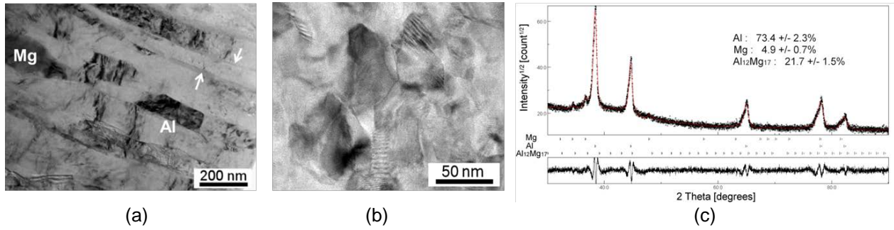
Fig. 3 TEM bright-field images taken at the Al-Mg disk edges after HPT for (a) 5 turns and (b) 10 turns and (c) the XRD profile with the MAUD estimation for the disk edge after 10 HPT turns [13].
