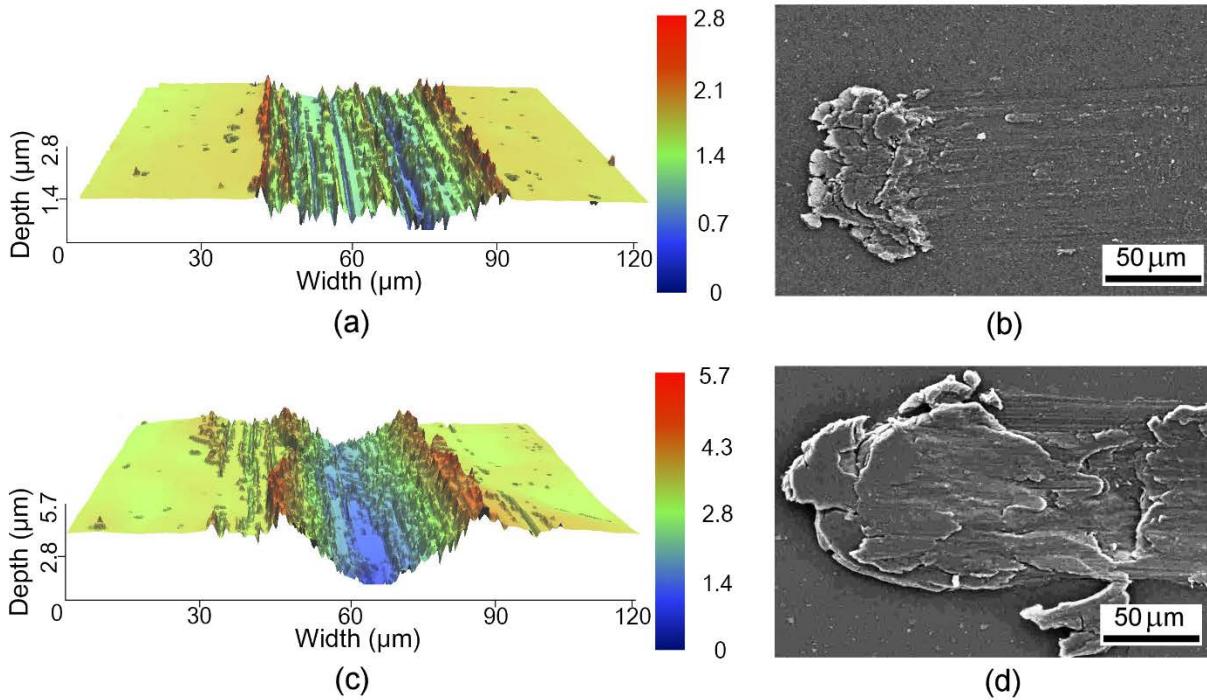
Fig. 8 Three-dimensional depth-sensing images at the vertical sections in the middle of the wear tracks (left) and the equivalent SEM micrographs of the worn surfaces (right) for (a) and (b) the MMNC at the disk edge in the Al-Mg system after HPT for 20 turns and (c) and (d) another MMNC at the disk edge after HPT and PDA: the detailed depth information is denoted by the color key beside each depth-sensing plot [16].
