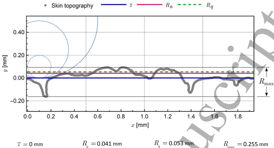
Figure 6. Surface characteristics of the skin sample used in this study: mean surface \bar{z} , surface roughness R_a , RMS roughness R_q and maximum peak-to-valley height R_{\max} .
