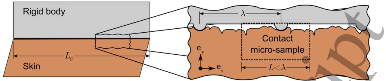
Figure 1. Schematic illustration of the rationale behind the contact homogenisation procedure used in this study. It consists of defining a representative section of the skin microstructure (length L ) together with a rigid surface featuring rigid hemi-spherical rigid asperities separated by a distance \lambda > L . At the macroscopic scale ( L_C ), assembly of these periodic structures (individually referred as contact micro-sample ) represent a macroscopic rigid body in contact with a macroscopic portion of skin.
