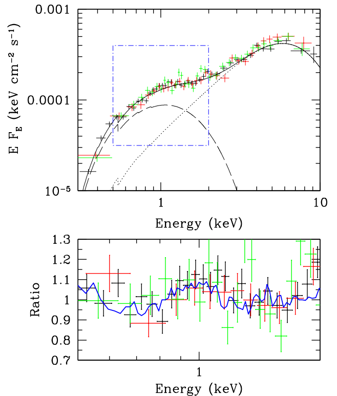
Figure 1. Upper panel: XMM-Newton spectral data points (PN: black, MOS1: red and MOS2: green) for P13 (re-binned for clarity). The best-fitting, unfolded model of TBABS*(DISKBB+NTHCOMP) is shown as a solid line (see Table 1 for parameters and 1 \sigma errors) with the DISKBB component shown as a dashed line and NTHCOMP as a dotted line. The blue, dot-dashed bounding box indicates the region of interest for the study of residuals to the model. Lower panel: 0.5-2 keV residuals to the best-fitting spectral model (same colour scheme as the upper panel). These cannot be adequately described by a constant at unity (null hypothesis probability < 0.05 ) but resemble the residuals seen in other ULXs (Middleton et al. 2015b). For reference, the blue line indicates the smoothed residuals of the ULX NGC 1313 X-1 (Middleton et al. 2015b) which have since been unambiguously resolved into emission and absorption features associated with a relativistically outflowing wind (Pinto et al. 2016; Walton et al. 2016a).
