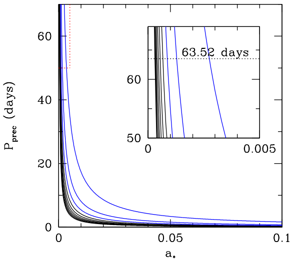
Figure 2. Precession period, P_{prec} , versus dimensionless spin parameter a_* . Using estimated wind parameters and T_{sph} from the X-ray spectrum as input (see Table 1), we determine the predicted precession period for a given compact object mass and spin. Masses shown in black are typical black hole masses (3-10 M_{\odot} in steps of 1 M_{\odot} ) and in blue are neutron star masses (1-3 M_{\odot} in steps of 1 M_{\odot} ). The inset shows a zoom-in of the region bound by the red dotted lines which allows the range of mass-spin values for the observed precession period of P13 (Motch et al. 2014, indicated by a horizontal dashed line) to be more clearly discerned.
