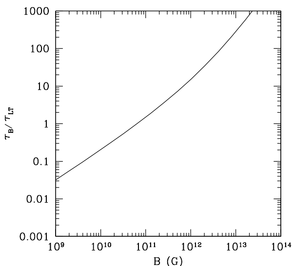
Figure 8. Ratio of magnetic torque (due to the interaction of the neutron star’s magnetic field with the disc - Lipunov & Shakura 1980) to the Lense-Thirring torque as a function of dipole field strength. Whilst it would appear that above a few \times 10^{10} G magnetic torques will dominate, we stress that this effect has only been studied in the thin disc regime which differs significantly from the super-critical regime and we expect the magnetic torque to be heavily diluted (see main text).
