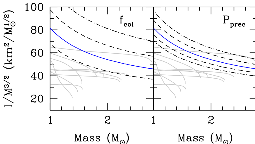
Figure 5. In the left-hand panel we show the impact of 5% (dashed) and 10% (dot-dashed) uncertainties on the limiting value of f_{col} , whilst in the right-hand panel we show the impact of uncertainties of 5 days (dashed) and 10 days (dot-dashed) in P_{prec} . In both cases we overlay the resulting moment-of-inertia curves on the theoretical EoS (see Figure 3 for details) and assume B = 1 \times 10^{12} G.
