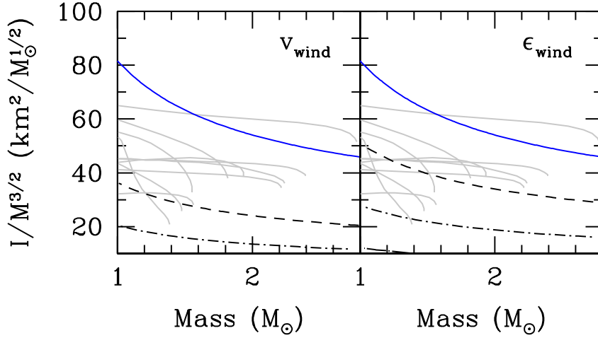
Figure 6. In the left-hand panel we show the impact of assuming wind velocities of 0.15c (dashed) and 0.2c (dot-dashed), whilst in the right-hand panel we show the impact of smaller values of \epsilon_{wind} of 0.4 (dashed), 0.3 (dot-dashed) and 0.2 (dot-dot-dashed). In both cases we overlay the resulting moment-of-inertia curves on the theoretical EoS (see Figure 3 for details) and assume B = 1 \times 10^{12} G.
