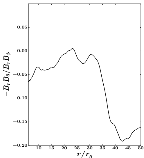
Figure 9. Ratio of the vertical (polar) and azimuthal components of Maxwell stress from the 3D RMHD simulation of Jiang et al. (2014). Clearly the ratio is far less than unity at all radii which could potentially place the warp within the spherisation radius, yet simulations have yet to encounter such a warp.
