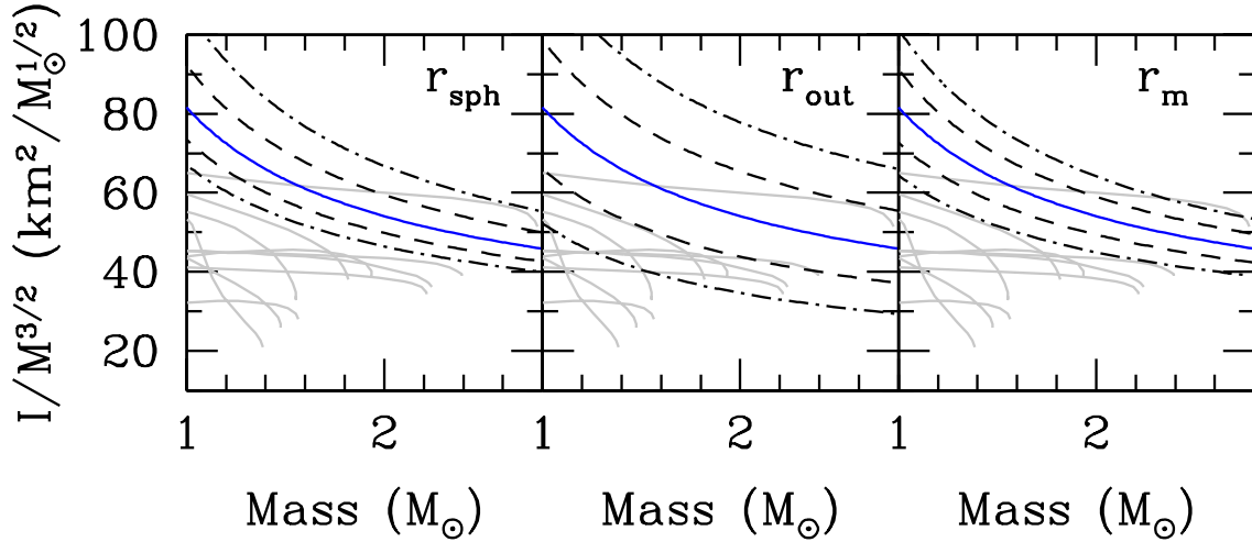
Figure 4. We plot the impact of 10% (dashed) and 20% (dot-dashed) systematic uncertainties on r_{sph} (left-hand panel), r_{out} (central panel) and r_m (right-hand panel). In all three cases we overlay the resulting moment-of-inertia curves on the theoretical EoS (see Figure 3 for details) and assume B = 1 \times 10^{12} G.
